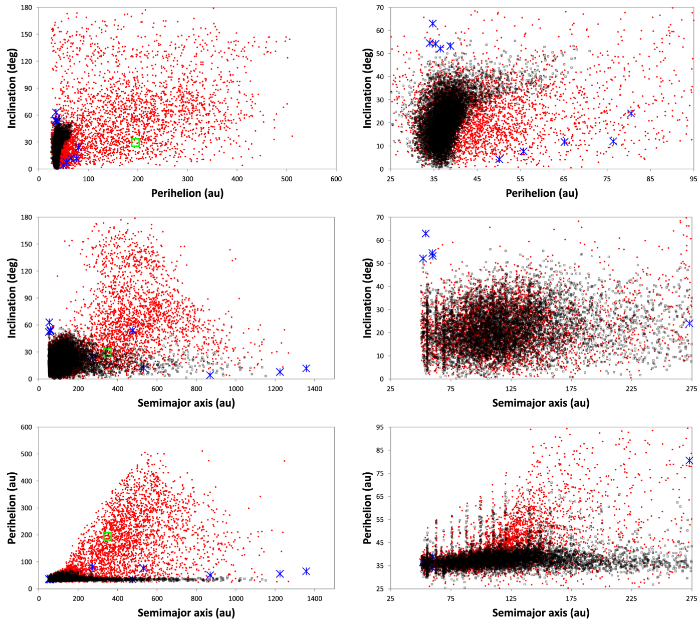
Figure 5. from Patryk Sofia Lykawka et al 2023 Astron. J. 166 doi:10.3847/1538-3881/aceaf0 https://dx.doi.org/10.3847/1538-3881/aceaf0 © 2023. The Author(s). Published by the American Astronomical Society.
