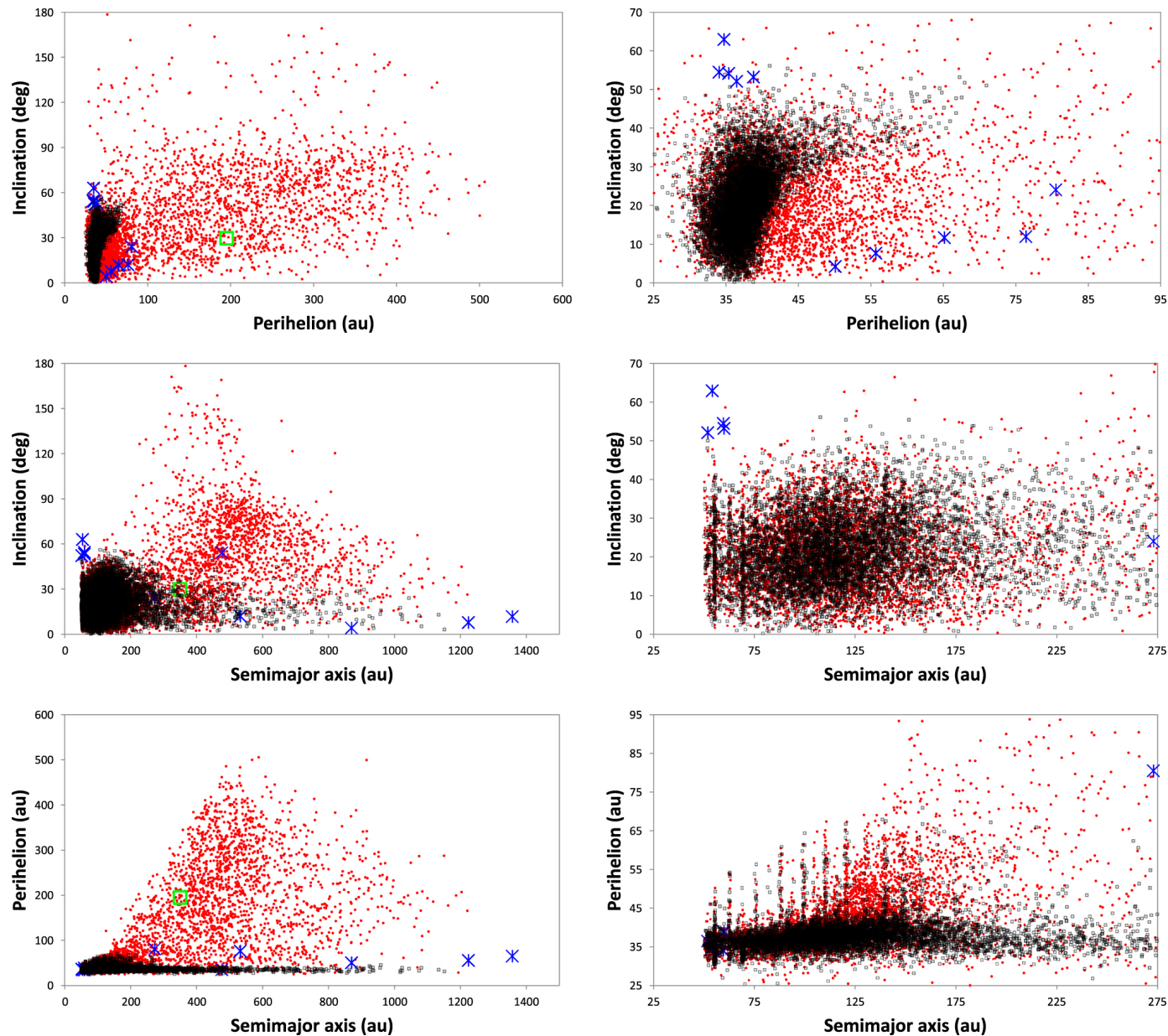
Figure 4. from Patryk Sofia Lykawka et al 2023 Astron. J. 166 doi:10.3847/1538-3881/aceaf0 https://dx.doi.org/10.3847/1538-3881/aceaf0 © 2023. The Author(s). Published by the American Astronomical Society.
