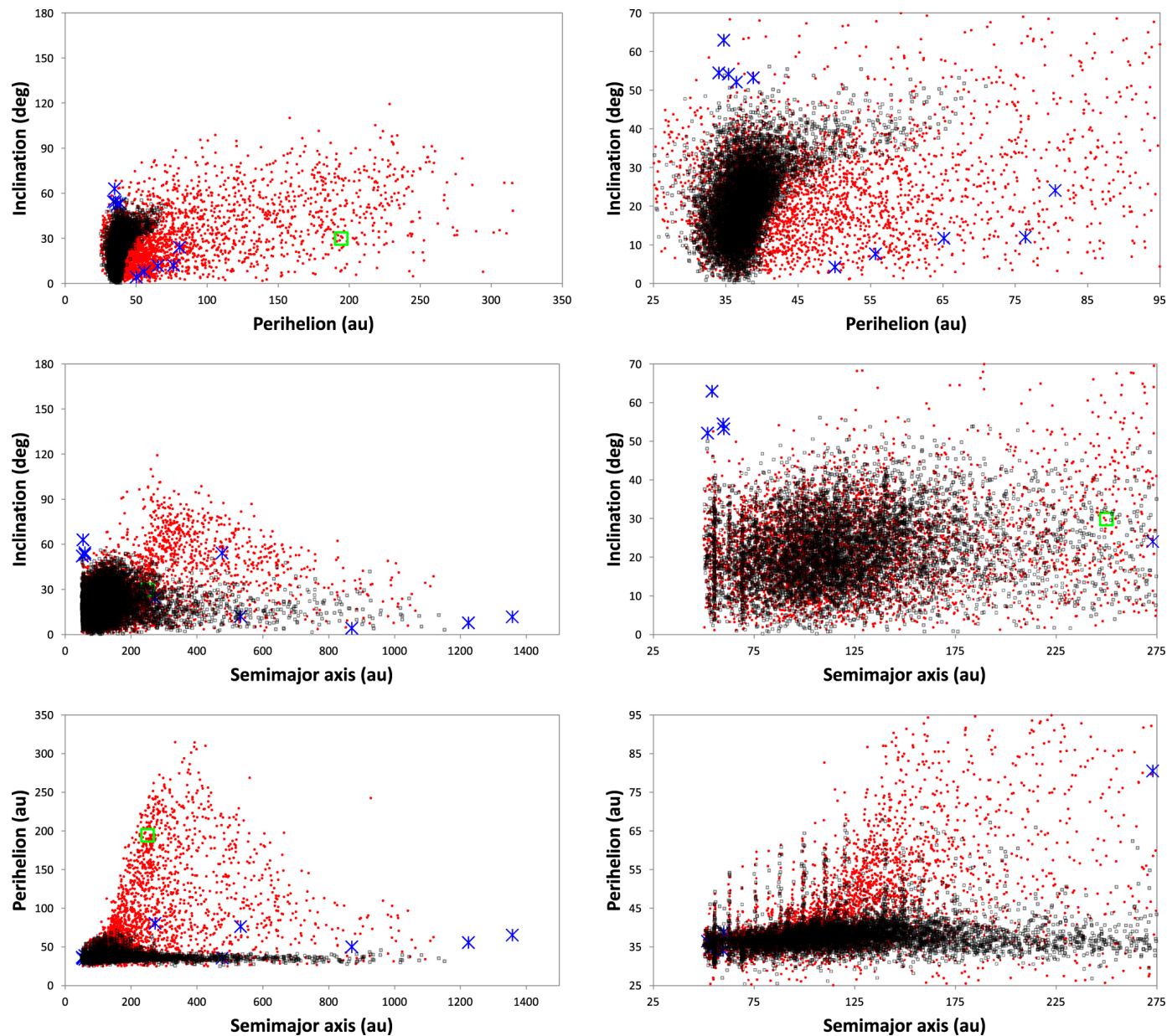
Figure 3. from Patryk Sofia Lykawka et al 2023 Astron. J. 166 doi:10.3847/1538-3881/aceaf0 https://dx.doi.org/10.3847/1538-3881/aceaf0 © 2023. The Author(s). Published by the American Astronomical Society.
