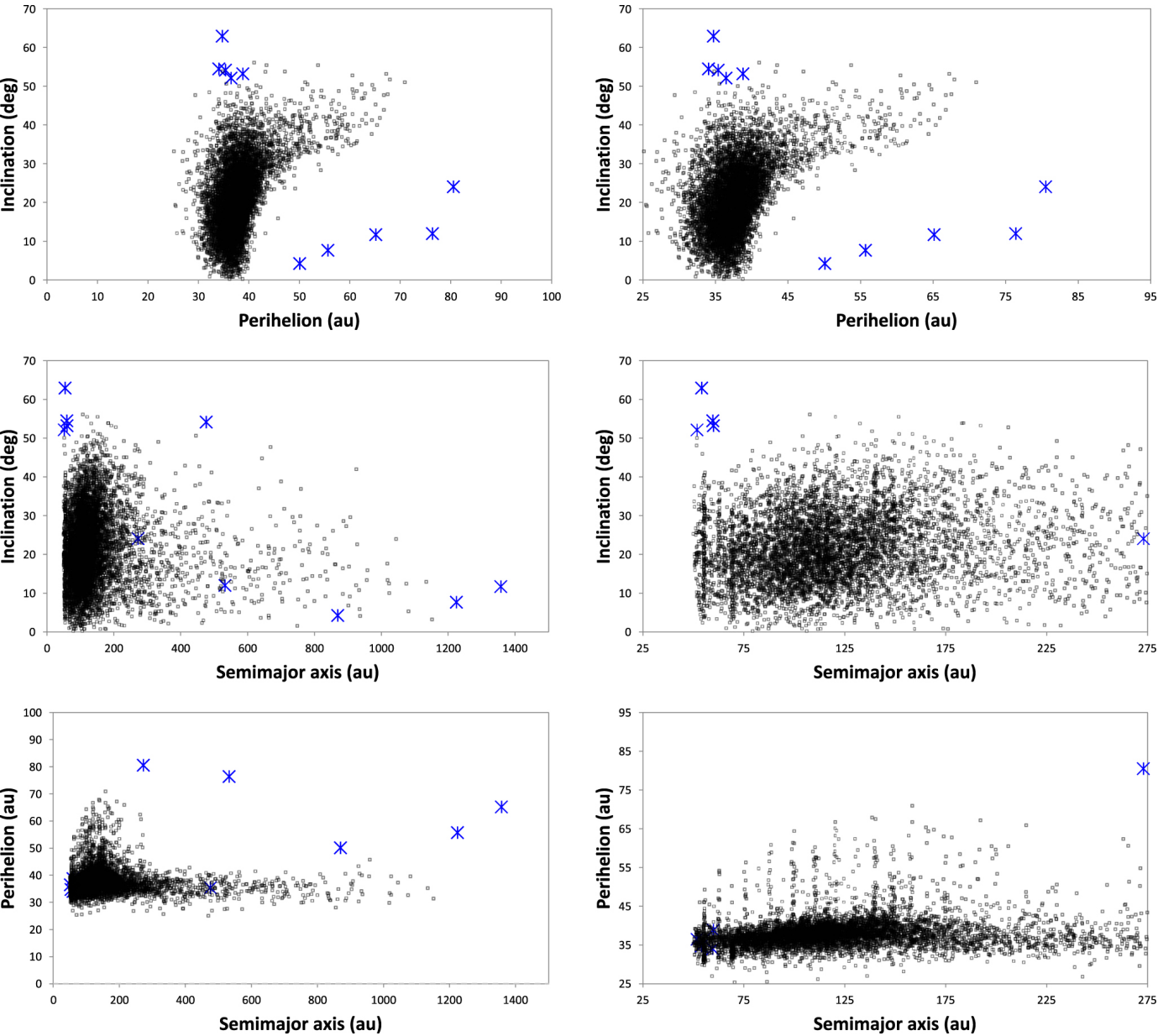
Figure 2. from Patryk Sofia Lykawka et al 2023 Astron. J. 166 doi:10.3847/1538-3881/aceaf0 https://dx.doi.org/10.3847/1538-3881/aceaf0 © 2023. The Author(s). Published by the American Astronomical Society.
