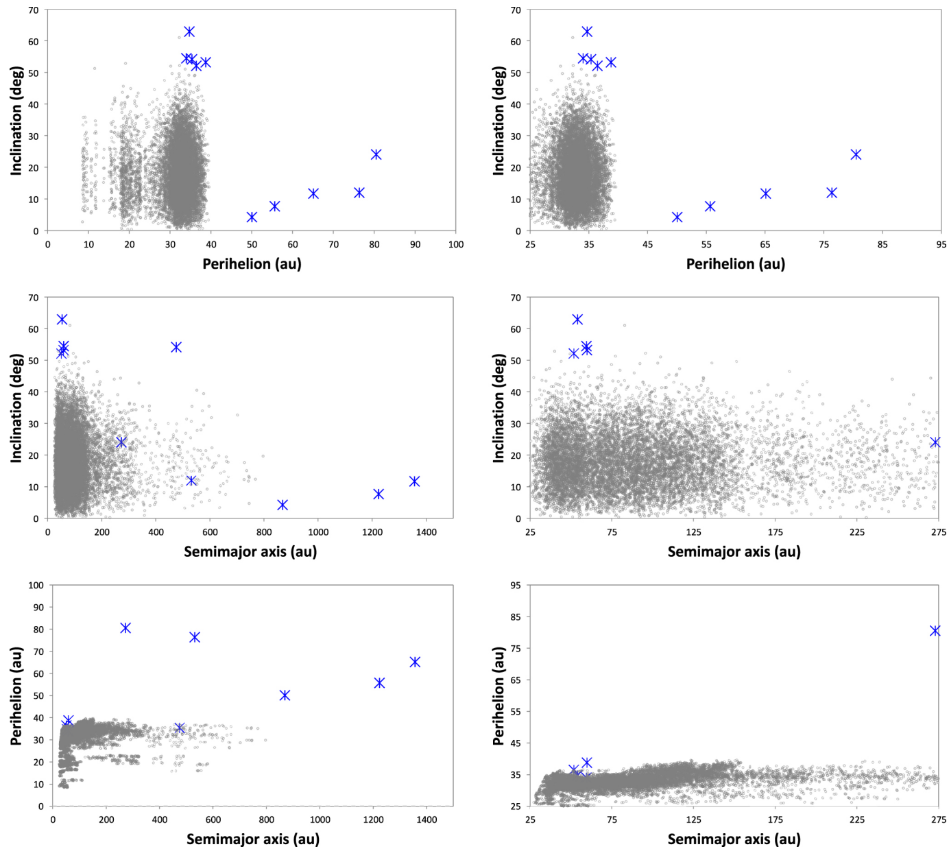
Figure 1. from Patryk Sofia Lykawka et al 2023 Astron. J. 166 doi:10.3847/1538-3881/aceaf0 https://dx.doi.org/10.3847/1538-3881/aceaf0 © 2023. The Author(s). Published by the American Astronomical Society.
