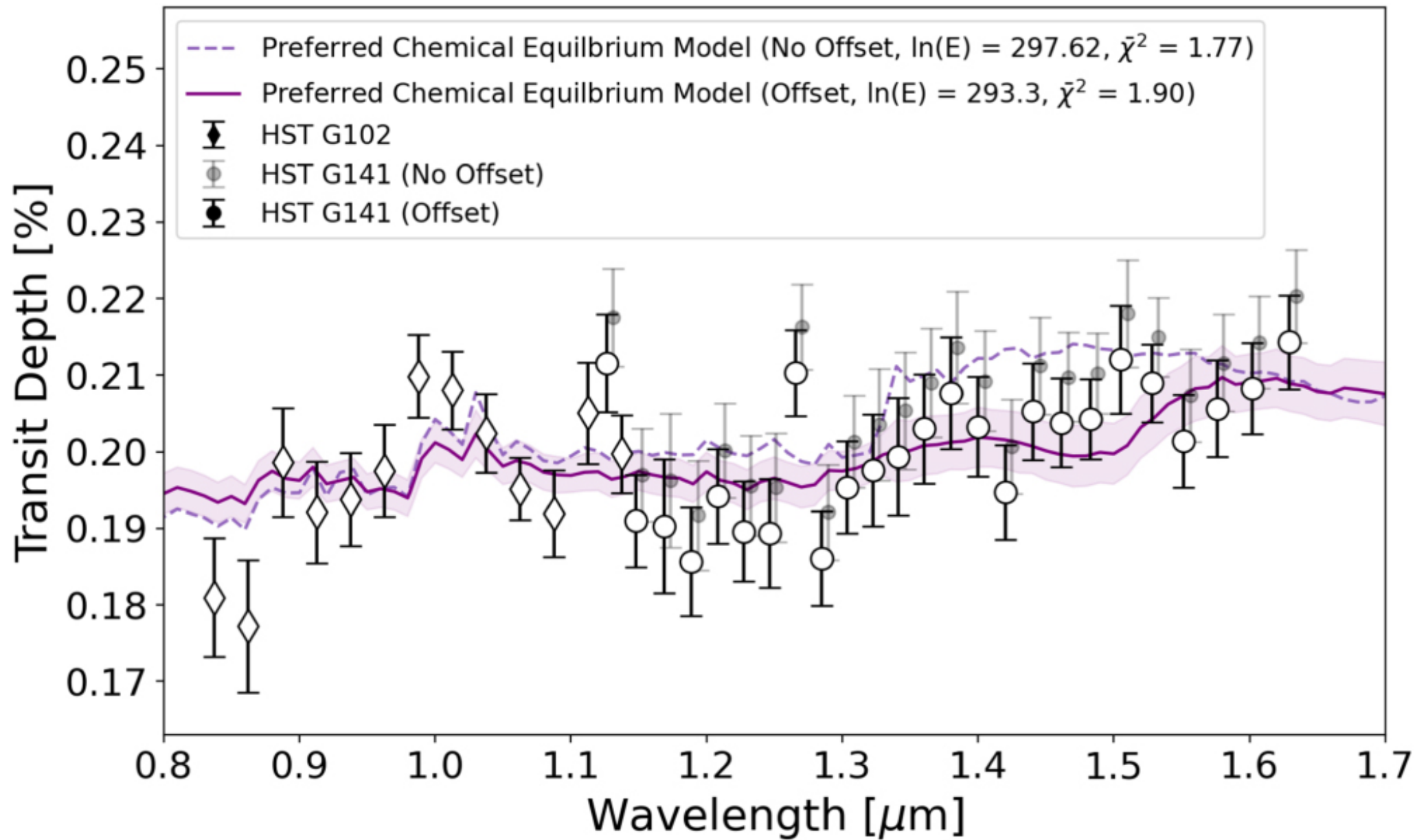
Figure 8. from Billy Edwards et al 2023 Astron. J. 166 doi:10.3847/1538-3881/acea77 https://dx.doi.org/10.3847/1538-3881/acea77 © 2023. The Author(s). Published by the American Astronomical Society.
