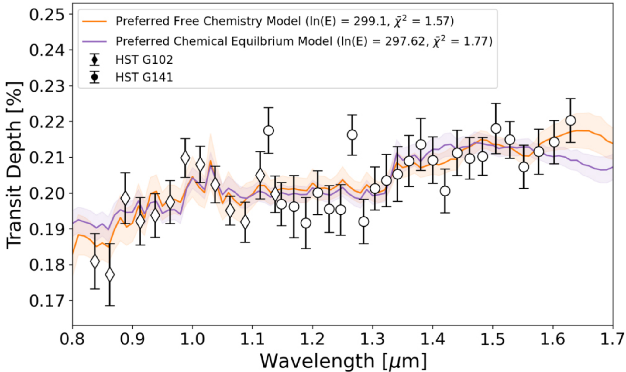
Figure 6. from Billy Edwards et al 2023 Astron. J. 166 doi:10.3847/1538-3881/acea77 https://dx.doi.org/10.3847/1538-3881/acea77 © 2023. The Author(s). Published by the American Astronomical Society.
