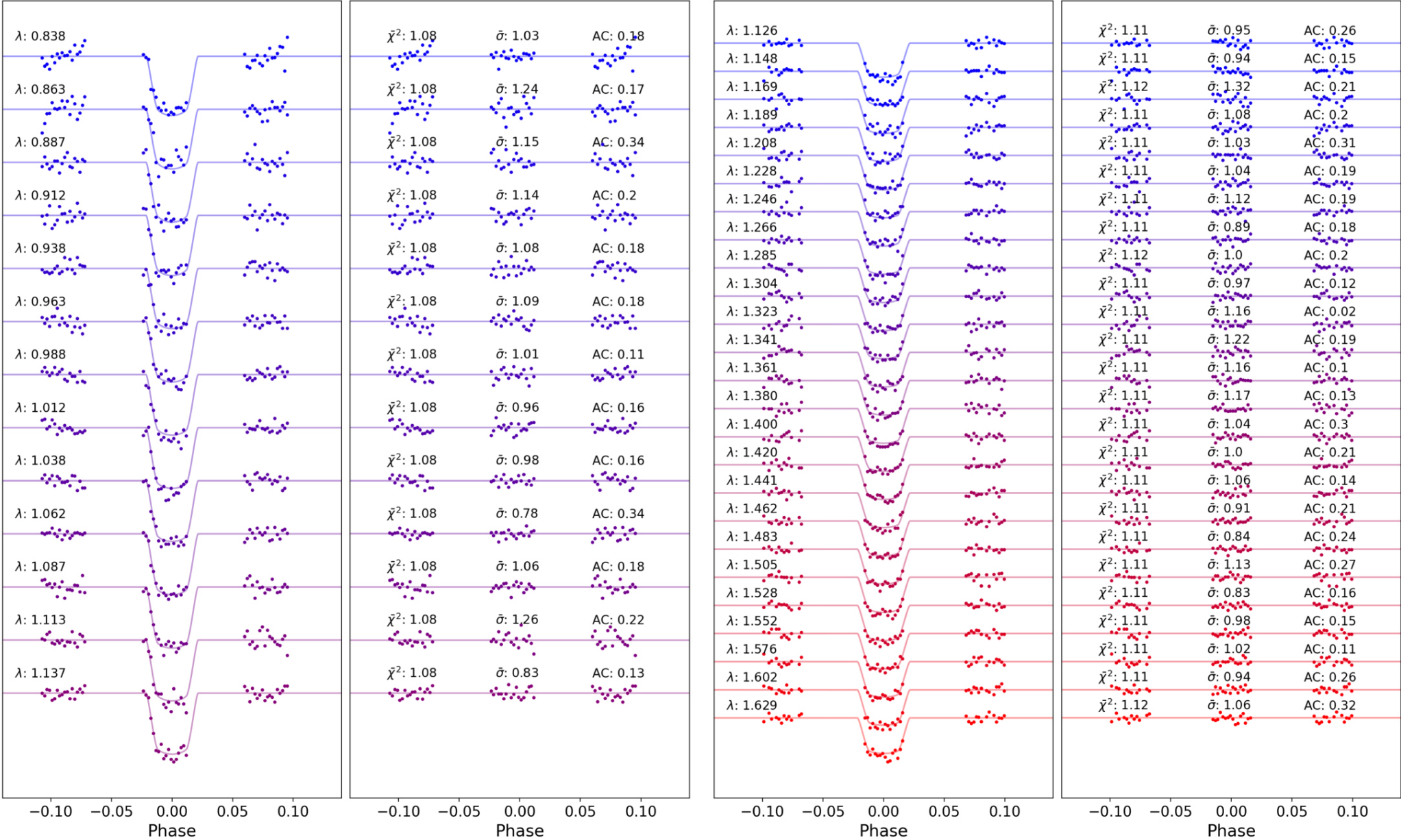
Figure 5. from Billy Edwards et al 2023 Astron. J. 166 doi:10.3847/1538-3881/acea77 https://dx.doi.org/10.3847/1538-3881/acea77 © 2023. The Author(s). Published by the American Astronomical Society.
