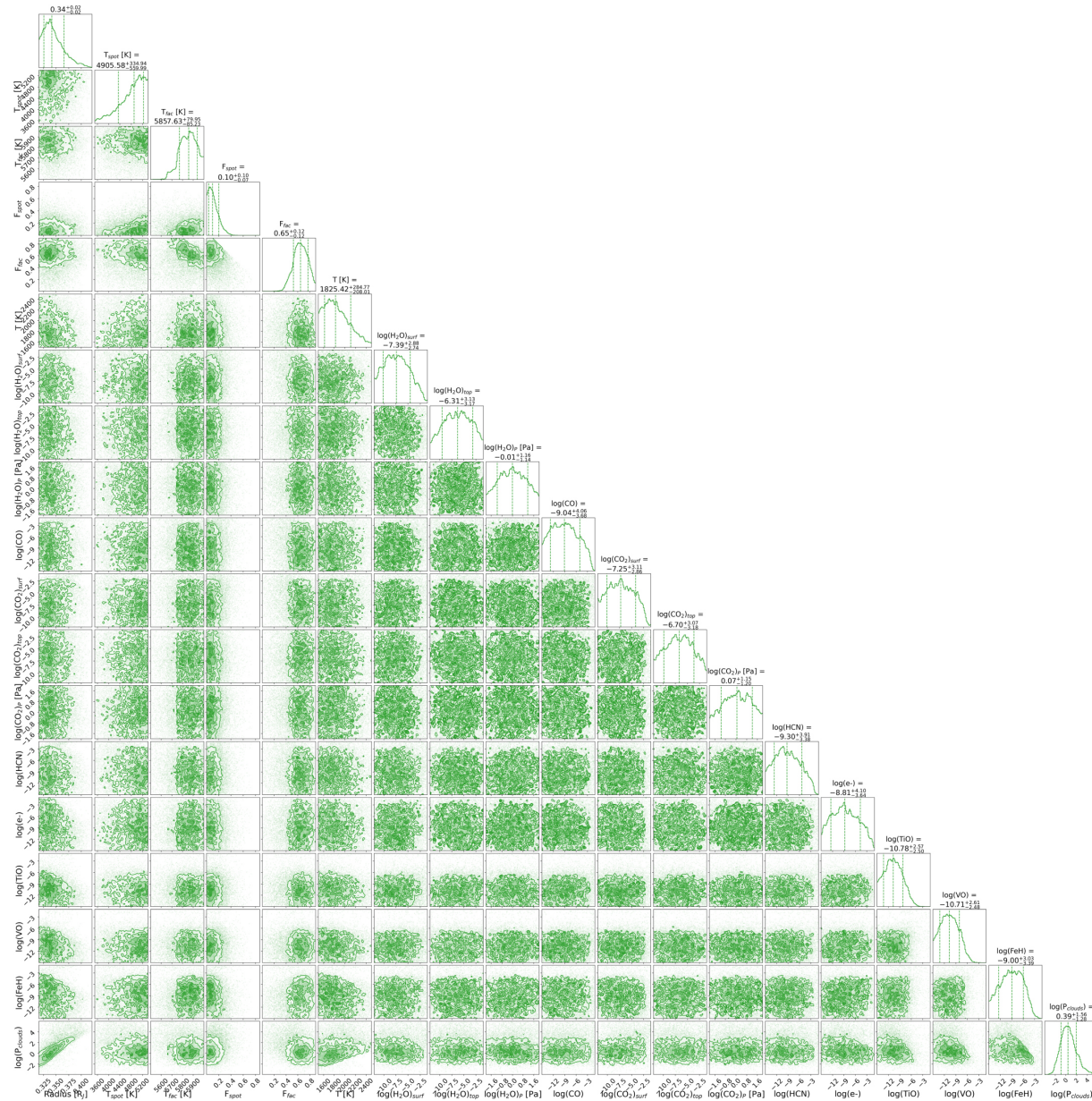
Figure 23. from Billy Edwards et al 2023 Astron. J. 166 doi:10.3847/1538-3881/acea77 https://dx.doi.org/10.3847/1538-3881/acea77 © 2023. The Author(s). Published by the American Astronomical Society.
