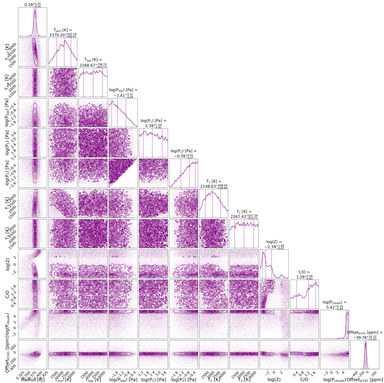
Figure 22. from Billy Edwards et al 2023 Astron. J. 166 doi:10.3847/1538-3881/acea77 https://dx.doi.org/10.3847/1538-3881/acea77 © 2023. The Author(s). Published by the American Astronomical Society.
