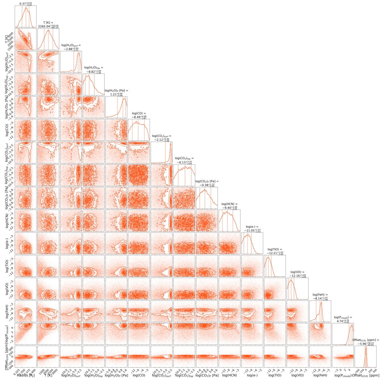
Figure 20. from Billy Edwards et al 2023 Astron. J. 166 doi:10.3847/1538-3881/acea77 https://dx.doi.org/10.3847/1538-3881/acea77 © 2023. The Author(s). Published by the American Astronomical Society.
