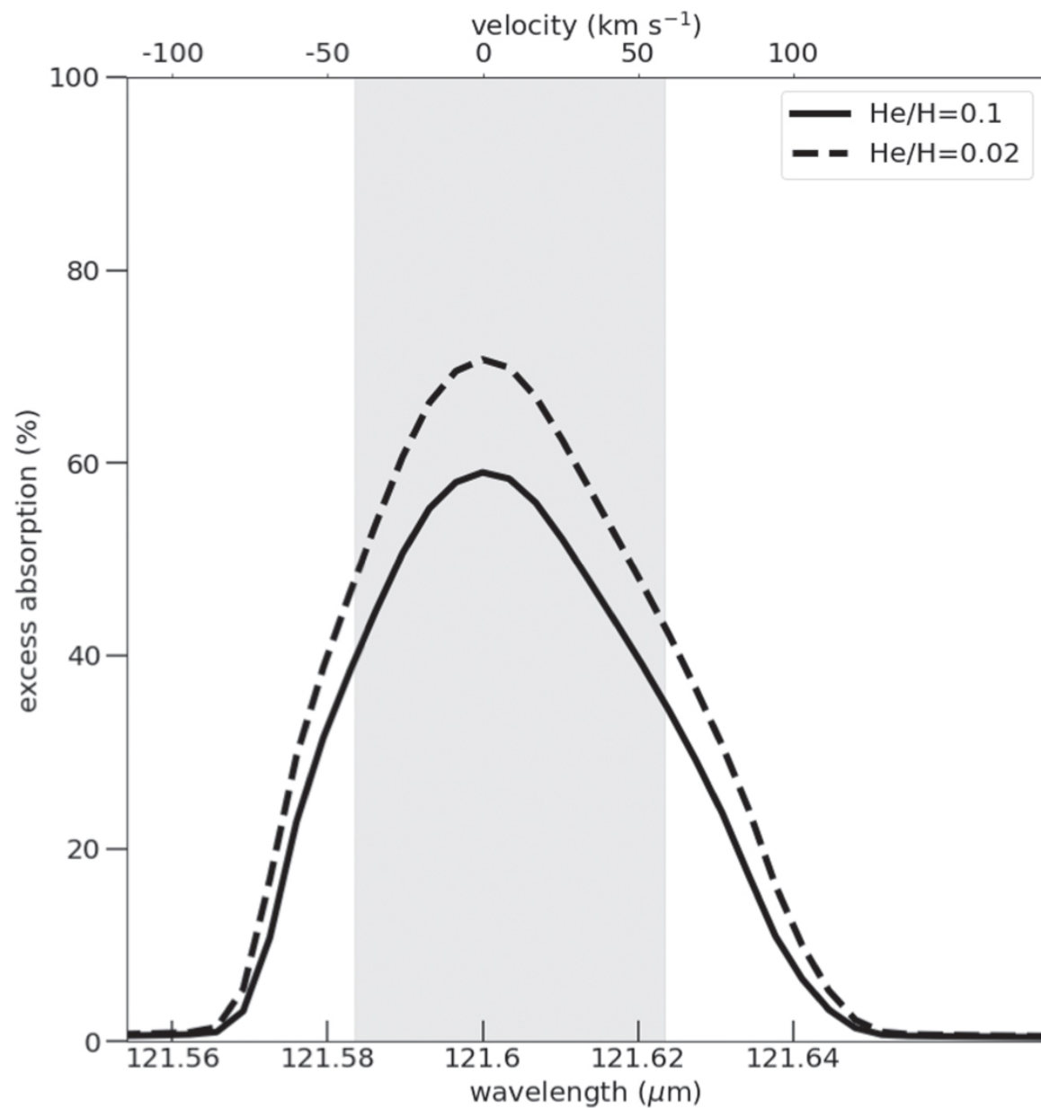
Figure 15. from Billy Edwards et al 2023 Astron. J. 166 doi:10.3847/1538-3881/acea77 https://dx.doi.org/10.3847/1538-3881/acea77 © 2023. The Author(s). Published by the American Astronomical Society.
