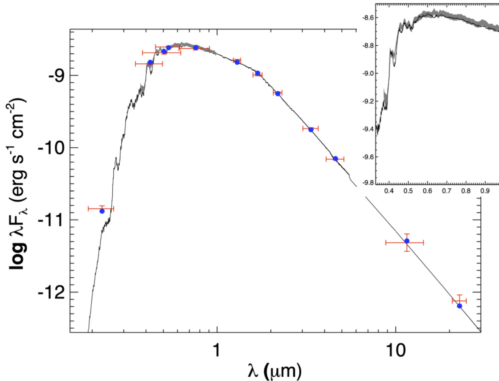
Figure 13. from Billy Edwards et al 2023 Astron. J. 166 doi:10.3847/1538-3881/acea77 https://dx.doi.org/10.3847/1538-3881/acea77 © 2023. The Author(s). Published by the American Astronomical Society.
