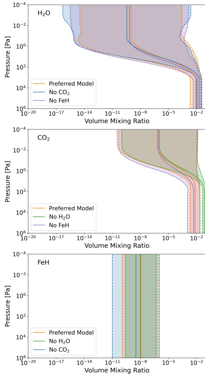
Figure 12. from Billy Edwards et al 2023 Astron. J. 166 doi:10.3847/1538-3881/acea77 https://dx.doi.org/10.3847/1538-3881/acea77 © 2023. The Author(s). Published by the American Astronomical Society.
