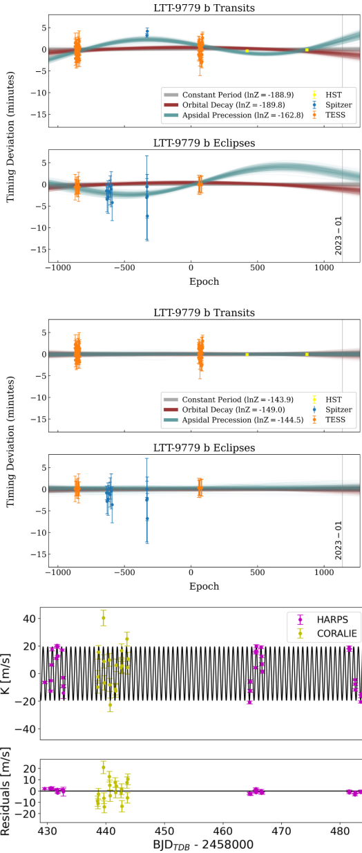
Figure 11. from Billy Edwards et al 2023 Astron. J. 166 doi:10.3847/1538-3881/acea77 https://dx.doi.org/10.3847/1538-3881/acea77 © 2023. The Author(s). Published by the American Astronomical Society.
