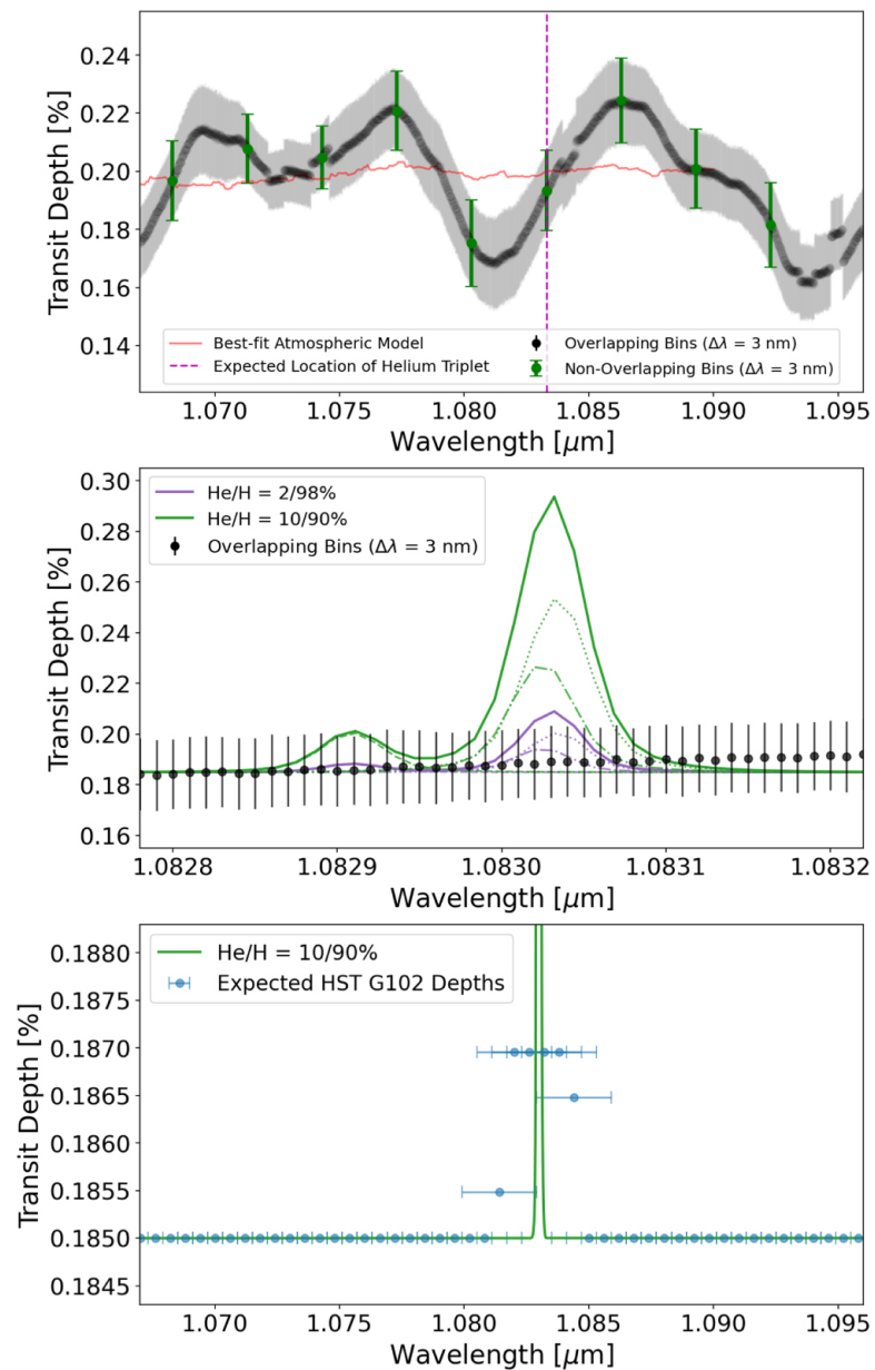
Figure 10. from Billy Edwards et al 2023 Astron. J. 166 doi:10.3847/1538-3881/acea77 https://dx.doi.org/10.3847/1538-3881/acea77 © 2023. The Author(s). Published by the American Astronomical Society.
