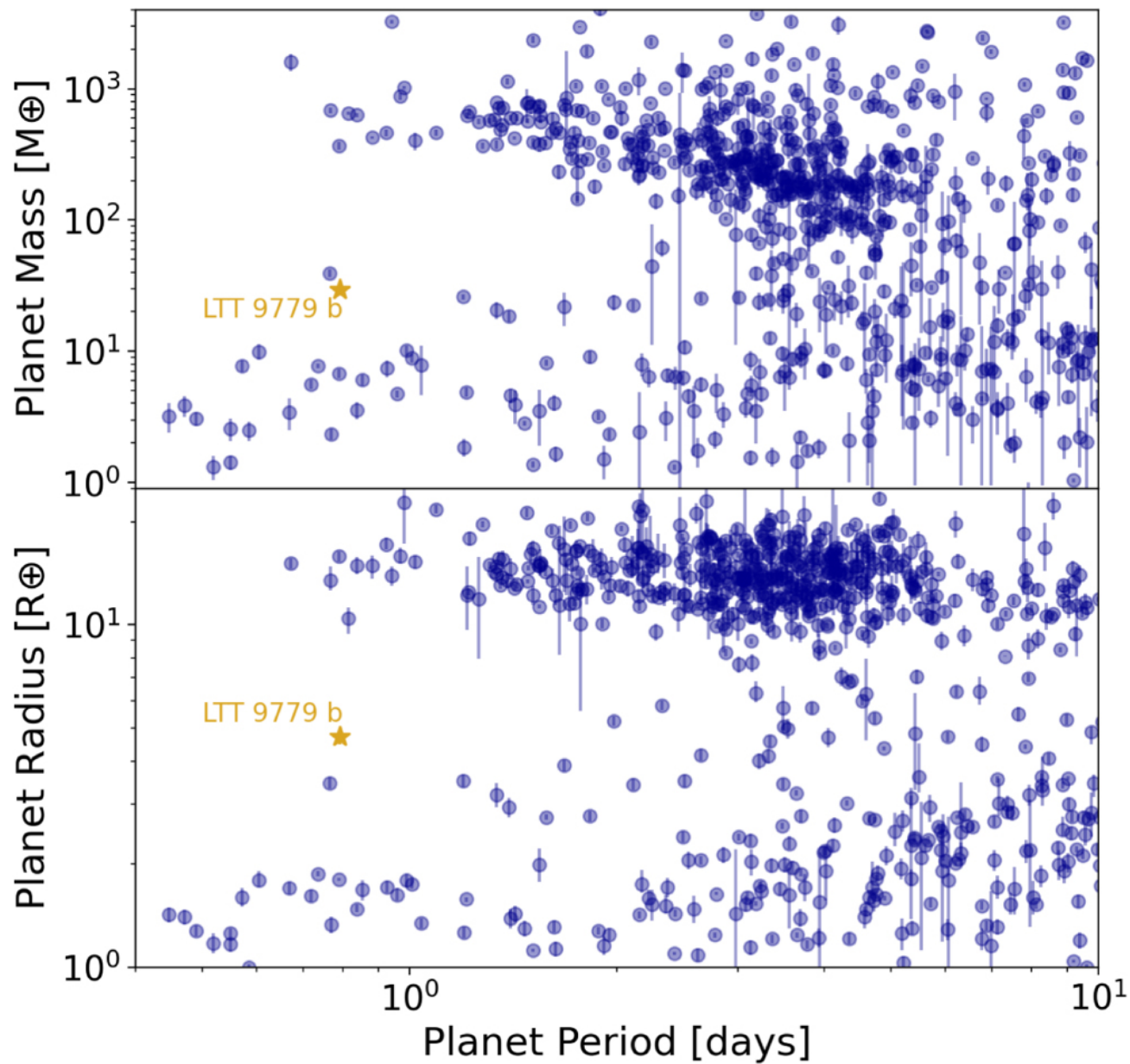
Figure 1. from Billy Edwards et al 2023 Astron. J. 166 doi:10.3847/1538-3881/acea77 https://dx.doi.org/10.3847/1538-3881/acea77 © 2023. The Author(s). Published by the American Astronomical Society.
