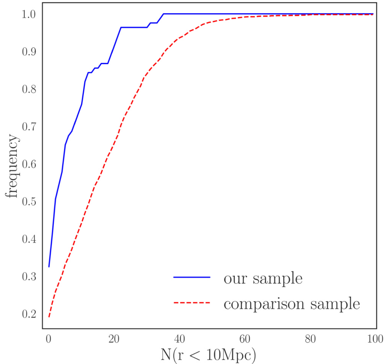
Figure 8. from Weiyu Ding et al 2023 Astron. J. 166 doi:10.3847/1538-3881/ace893 https://dx.doi.org/10.3847/1538-3881/ace893 © 2023. The Author(s). Published by the American Astronomical Society.
