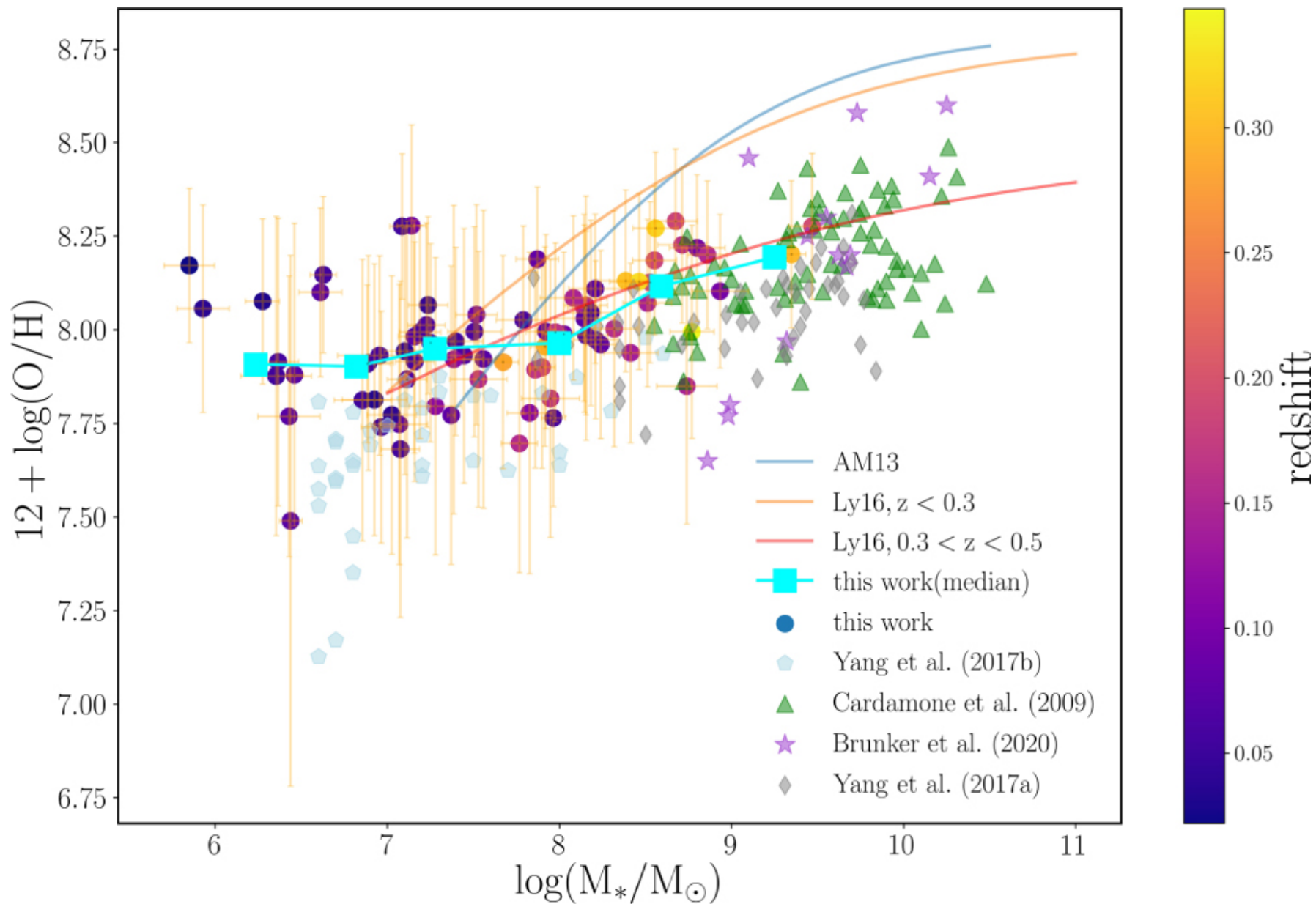
Figure 7. from Weiyu Ding et al 2023 Astron. J. 166 doi:10.3847/1538-3881/ace893 https://dx.doi.org/10.3847/1538-3881/ace893 © 2023. The Author(s). Published by the American Astronomical Society.
