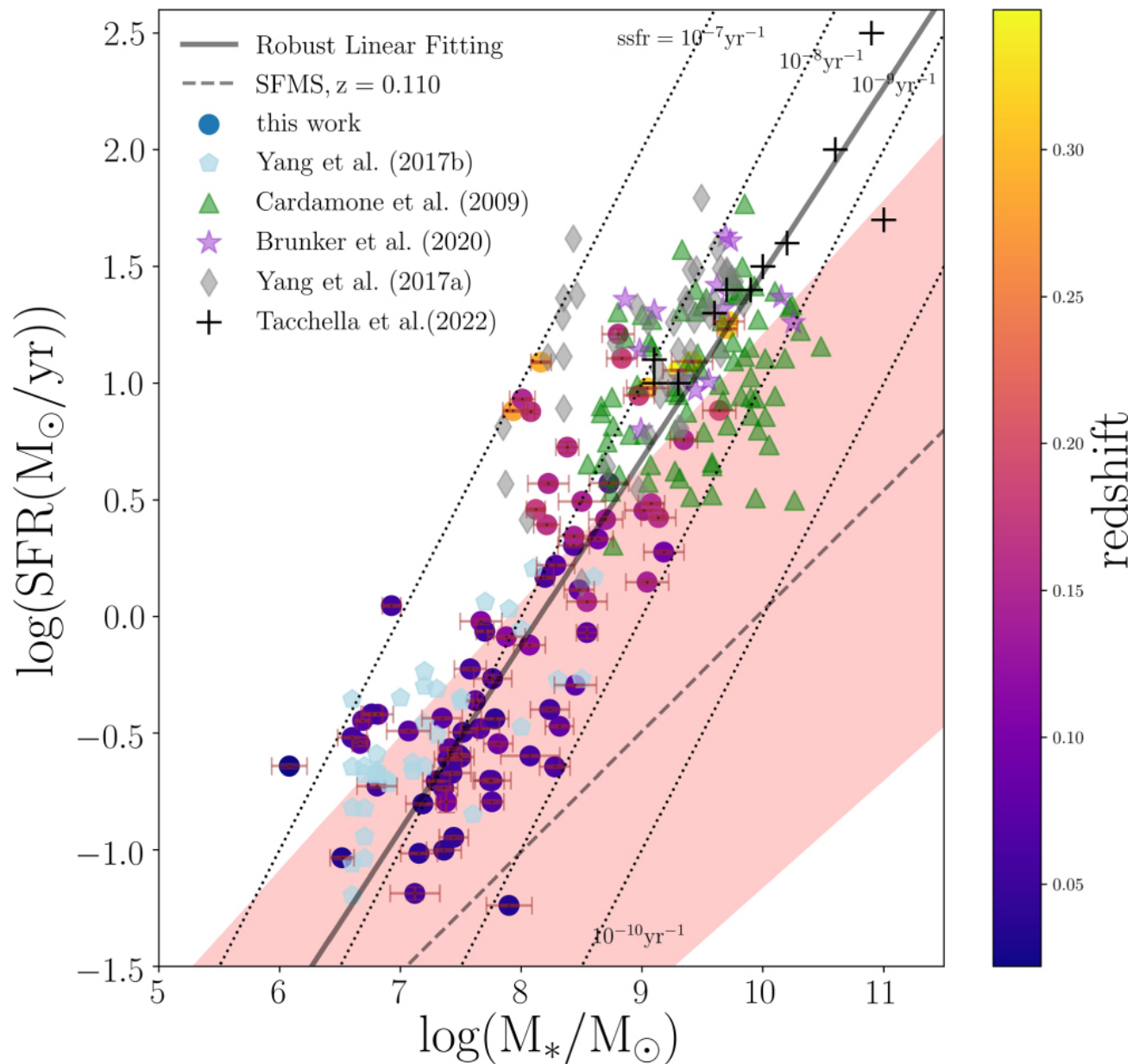
Figure 6. from Weiyu Ding et al 2023 Astron. J. 166 doi:10.3847/1538-3881/ace893 https://dx.doi.org/10.3847/1538-3881/ace893 © 2023. The Author(s). Published by the American Astronomical Society.
