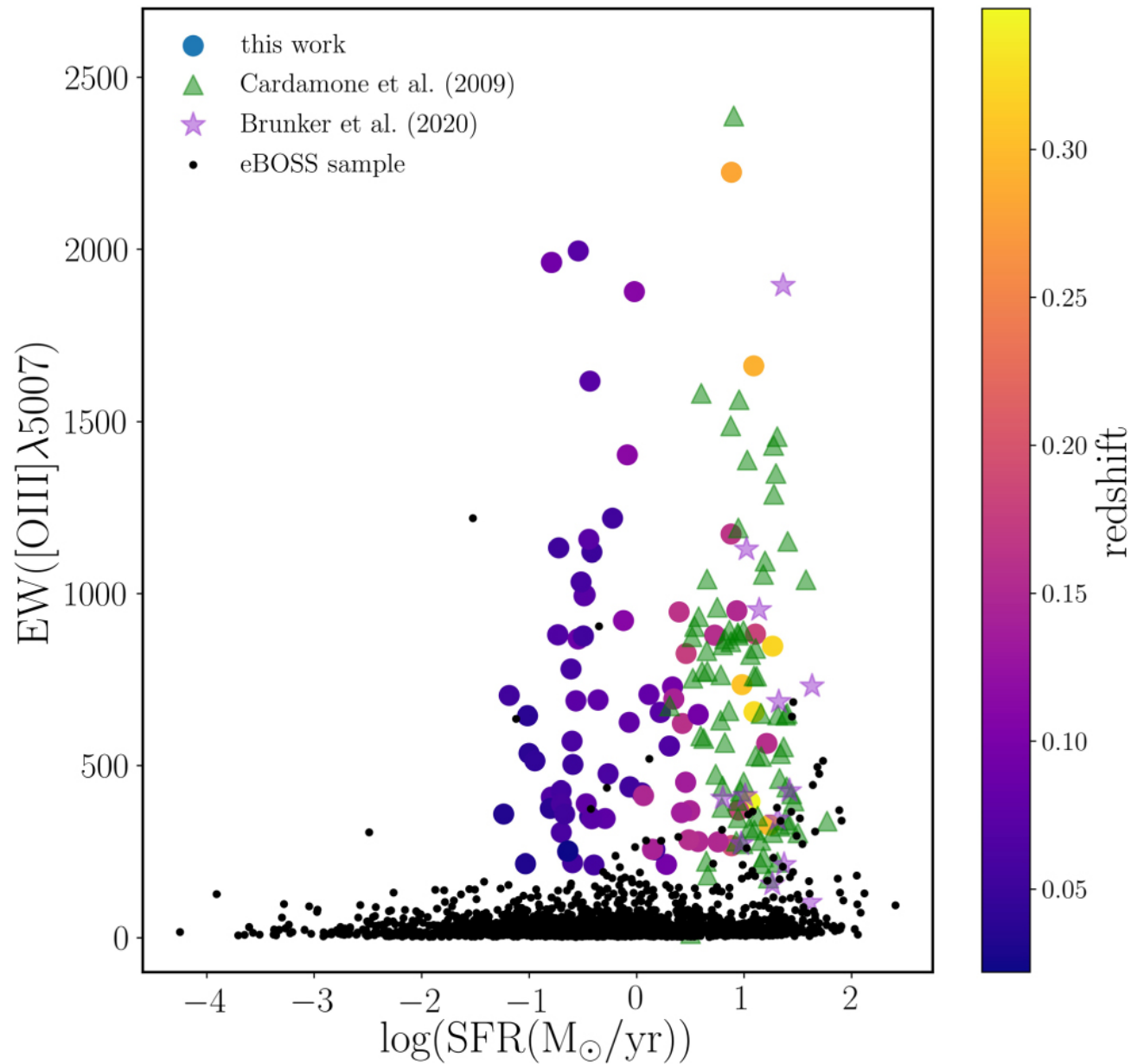
Figure 5. from Weiyu Ding et al 2023 Astron. J. 166 doi:10.3847/1538-3881/ace893 https://dx.doi.org/10.3847/1538-3881/ace893 © 2023. The Author(s). Published by the American Astronomical Society.
