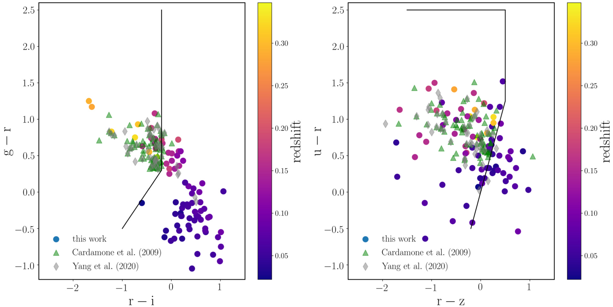
Figure 3. from Weiyu Ding et al 2023 Astron. J. 166 doi:10.3847/1538-3881/ace893 https://dx.doi.org/10.3847/1538-3881/ace893 © 2023. The Author(s). Published by the American Astronomical Society.
