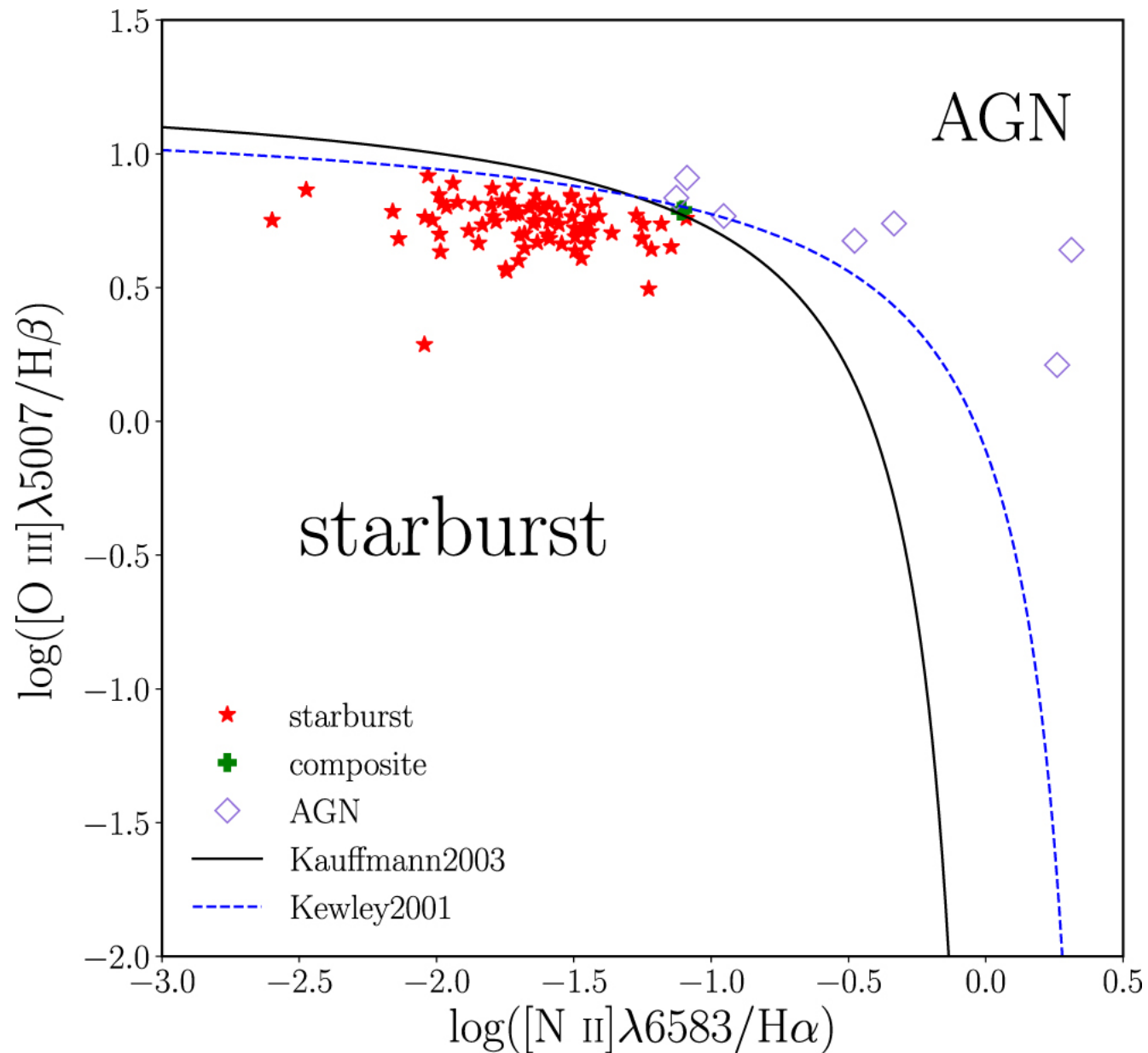
Figure 2. from Weiyu Ding et al 2023 Astron. J. 166 doi:10.3847/1538-3881/ace893 https://dx.doi.org/10.3847/1538-3881/ace893 © 2023. The Author(s). Published by the American Astronomical Society.
