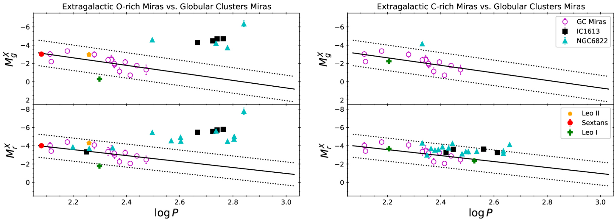
Figure 9. from C.-C. Ngeow et al 2023 Astron. J. 166 doi:10.3847/1538-3881/ace7b4 https://dx.doi.org/10.3847/1538-3881/ace7b4 © 2023. The Author(s). Published by the American Astronomical Society.
