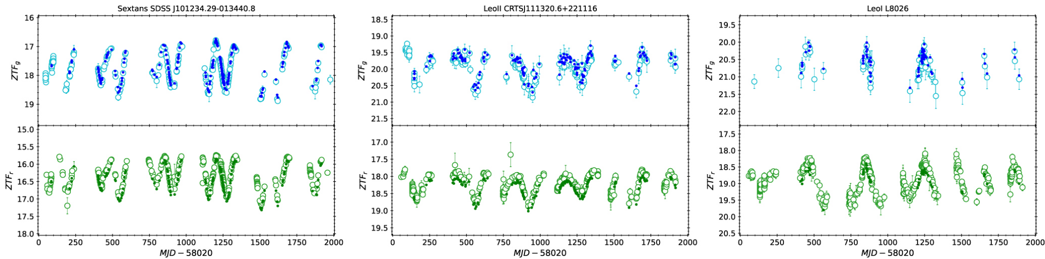
Figure 8. from C.-C. Ngeow et al 2023 Astron. J. 166 doi:10.3847/1538-3881/ace7b4 https://dx.doi.org/10.3847/1538-3881/ace7b4 © 2023. The Author(s). Published by the American Astronomical Society.
