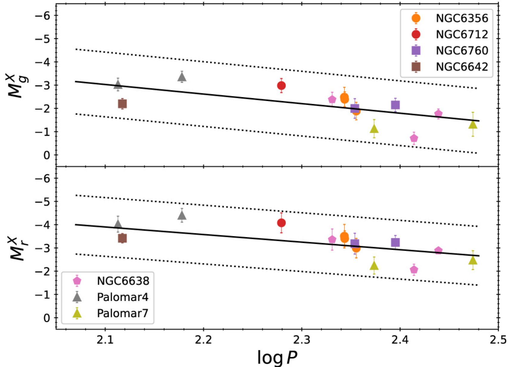
Figure 6. from C.-C. Ngeow et al 2023 Astron. J. 166 doi:10.3847/1538-3881/ace7b4 https://dx.doi.org/10.3847/1538-3881/ace7b4 © 2023. The Author(s). Published by the American Astronomical Society.
