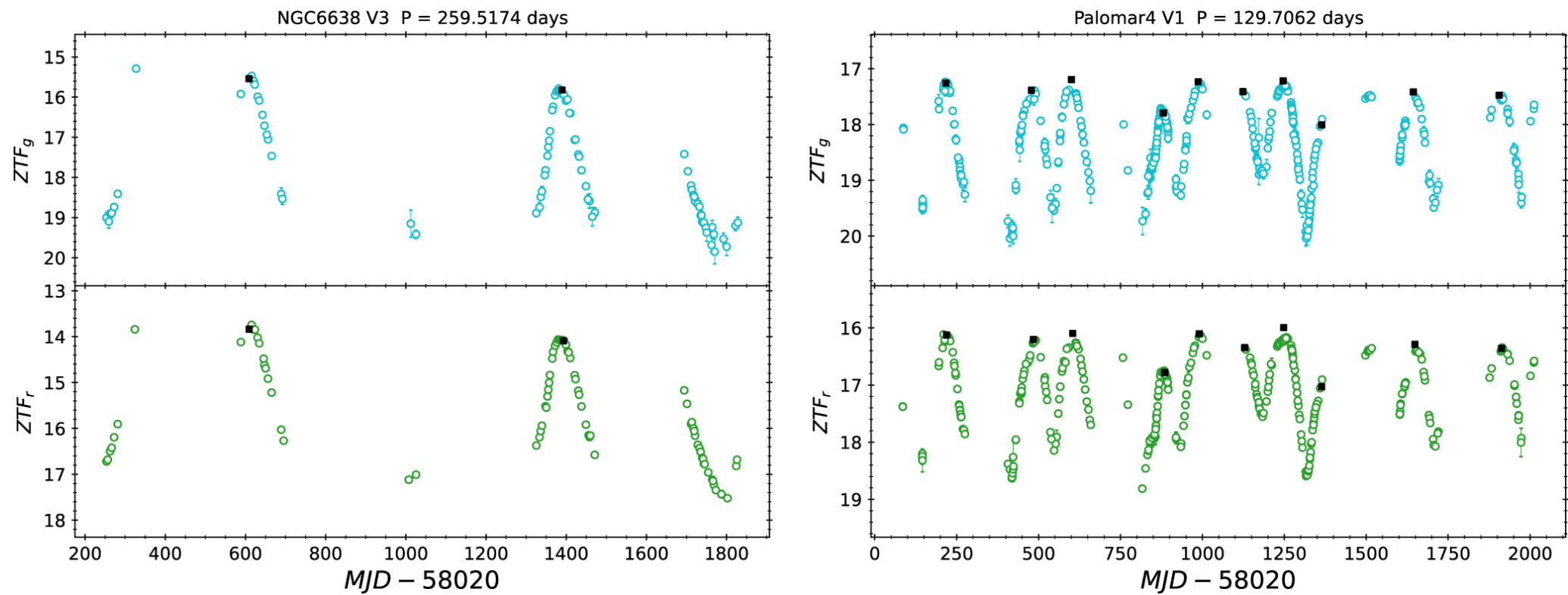
Figure 5. from C.-C. Ngeow et al 2023 Astron. J. 166 doi:10.3847/1538-3881/ace7b4 https://dx.doi.org/10.3847/1538-3881/ace7b4 © 2023. The Author(s). Published by the American Astronomical Society.
