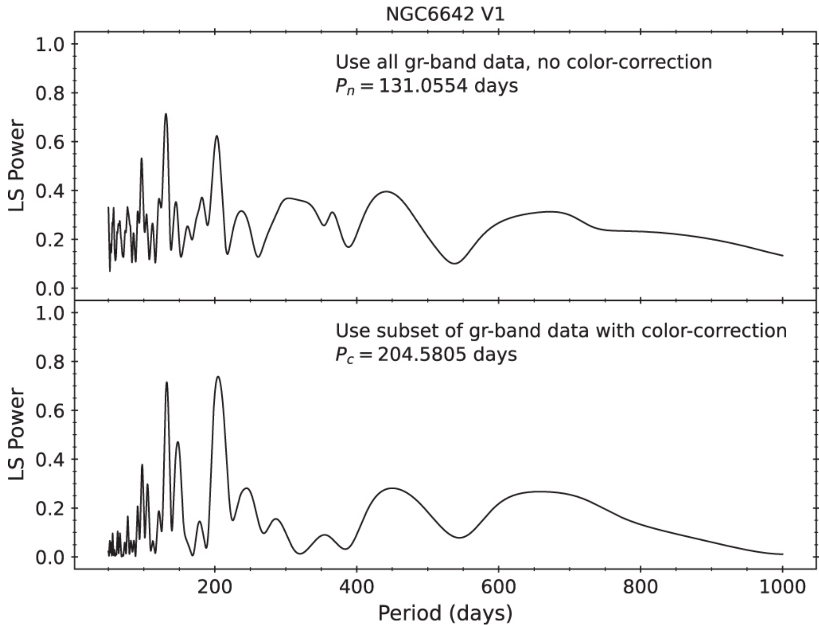
Figure 3. from C.-C. Ngeow et al 2023 Astron. J. 166 doi:10.3847/1538-3881/ace7b4 https://dx.doi.org/10.3847/1538-3881/ace7b4 © 2023. The Author(s). Published by the American Astronomical Society.
