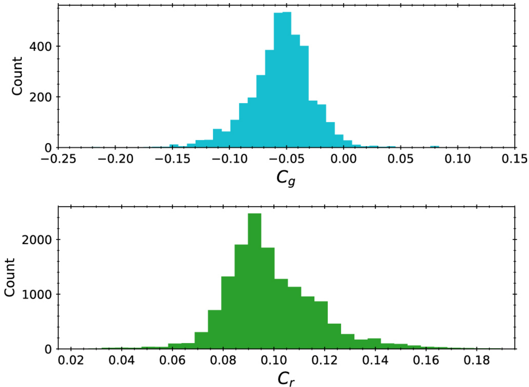
Figure 1. from C.-C. Ngeow et al 2023 Astron. J. 166 doi:10.3847/1538-3881/ace7b4 https://dx.doi.org/10.3847/1538-3881/ace7b4 © 2023. The Author(s). Published by the American Astronomical Society.
