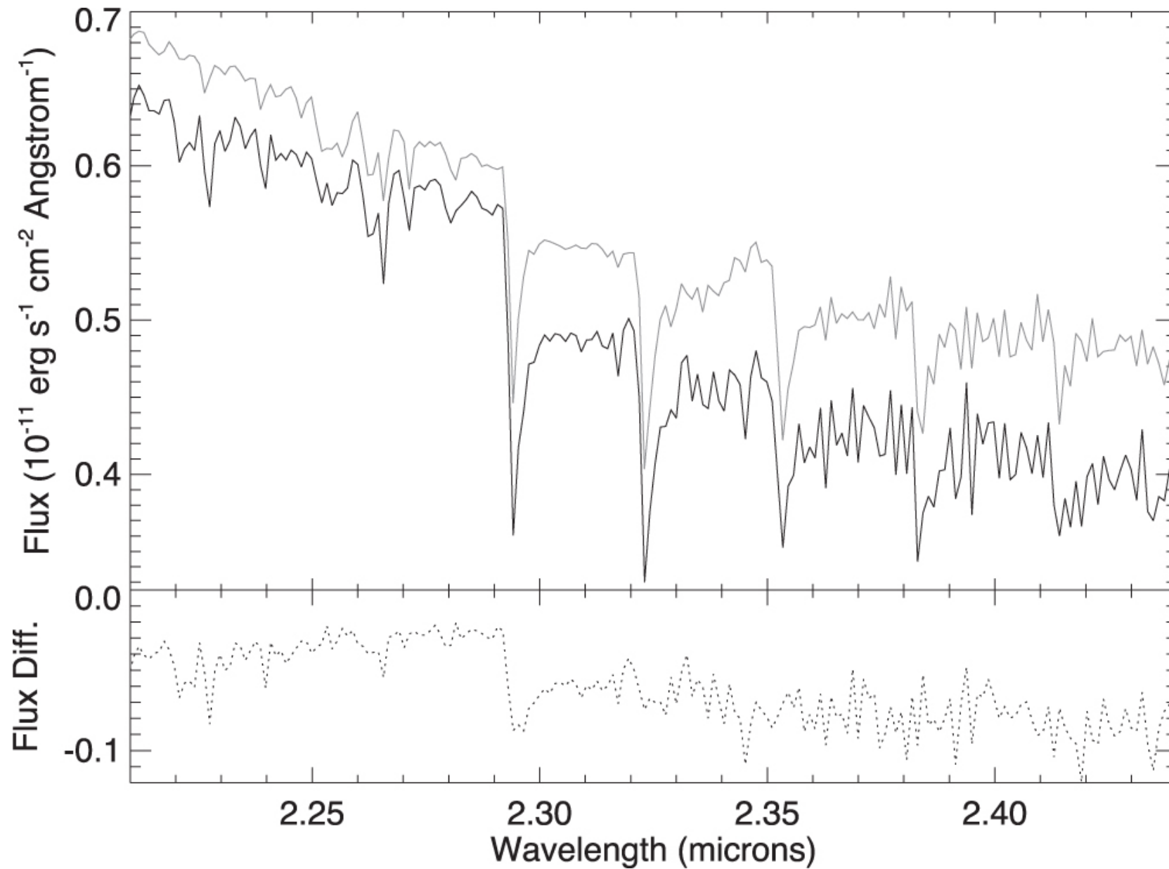
Figure 8. from Narsireddy Anugu et al 2023 Astron. J. 166 doi:10.3847/1538-3881/ace59d https://dx.doi.org/10.3847/1538-3881/ace59d © 2023. The Author(s). Published by the American Astronomical Society.
