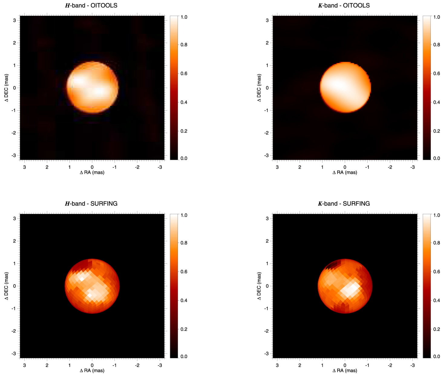
Figure 6. from Narsireddy Anugu et al 2023 Astron. J. 166 doi:10.3847/1538-3881/ace59d https://dx.doi.org/10.3847/1538-3881/ace59d © 2023. The Author(s). Published by the American Astronomical Society.
