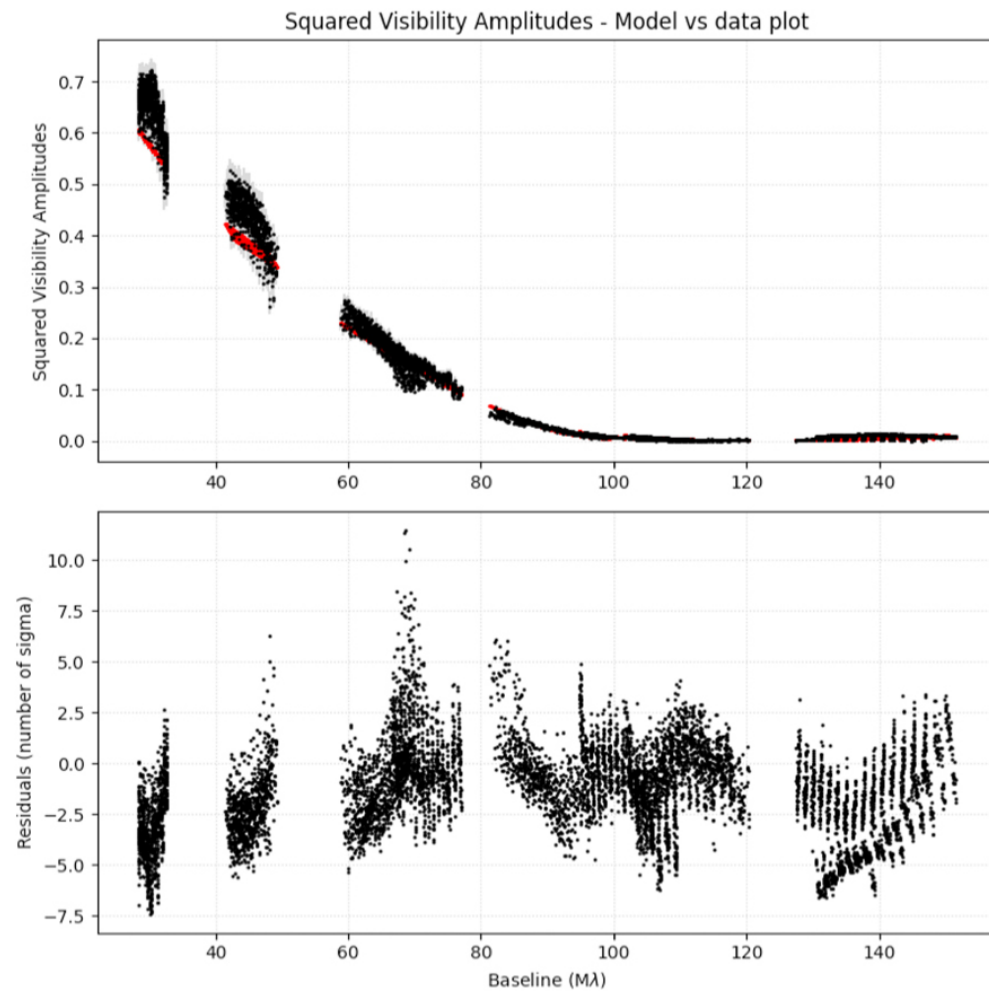
Figure 4. from Narsireddy Anugu et al 2023 Astron. J. 166 doi:10.3847/1538-3881/ace59d https://dx.doi.org/10.3847/1538-3881/ace59d © 2023. The Author(s). Published by the American Astronomical Society.
