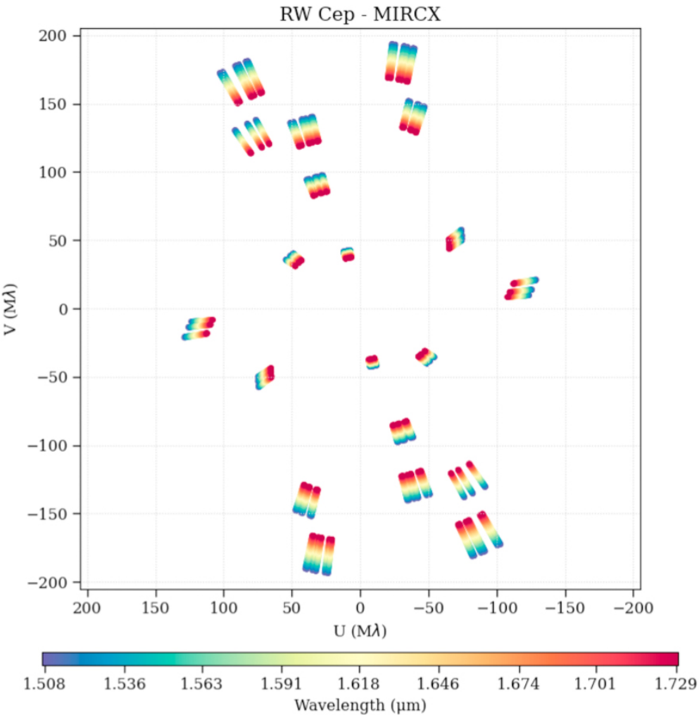
Figure 2. from Narsireddy Anugu et al 2023 Astron. J. 166 doi:10.3847/1538-3881/ace59d https://dx.doi.org/10.3847/1538-3881/ace59d © 2023. The Author(s). Published by the American Astronomical Society.
