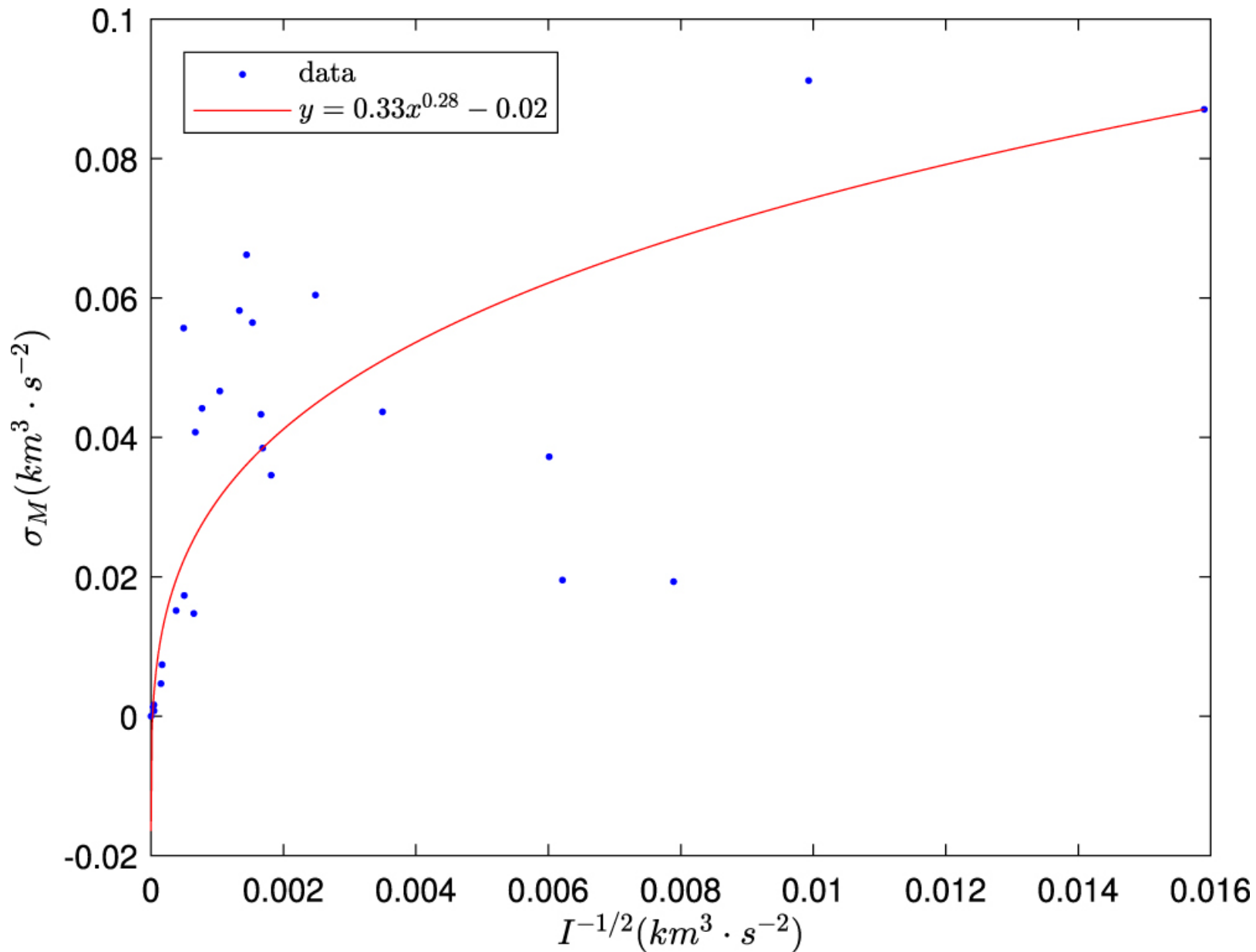
Figure 5. from Fan Li et al 2023 Astron. J. 166 doi:10.3847/1538-3881/ace52b https://dx.doi.org/10.3847/1538-3881/ace52b © 2023. The Author(s). Published by the American Astronomical Society.
