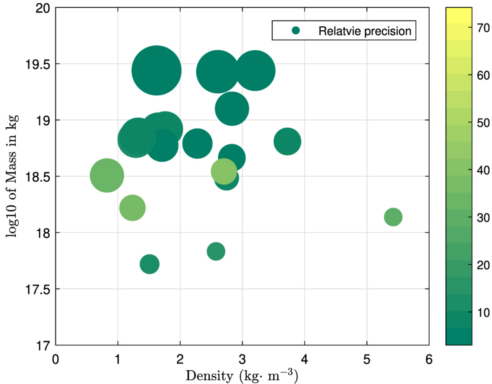
Figure 4. from Fan Li et al 2023 Astron. J. 166 doi:10.3847/1538-3881/ace52b https://dx.doi.org/10.3847/1538-3881/ace52b © 2023. The Author(s). Published by the American Astronomical Society.
