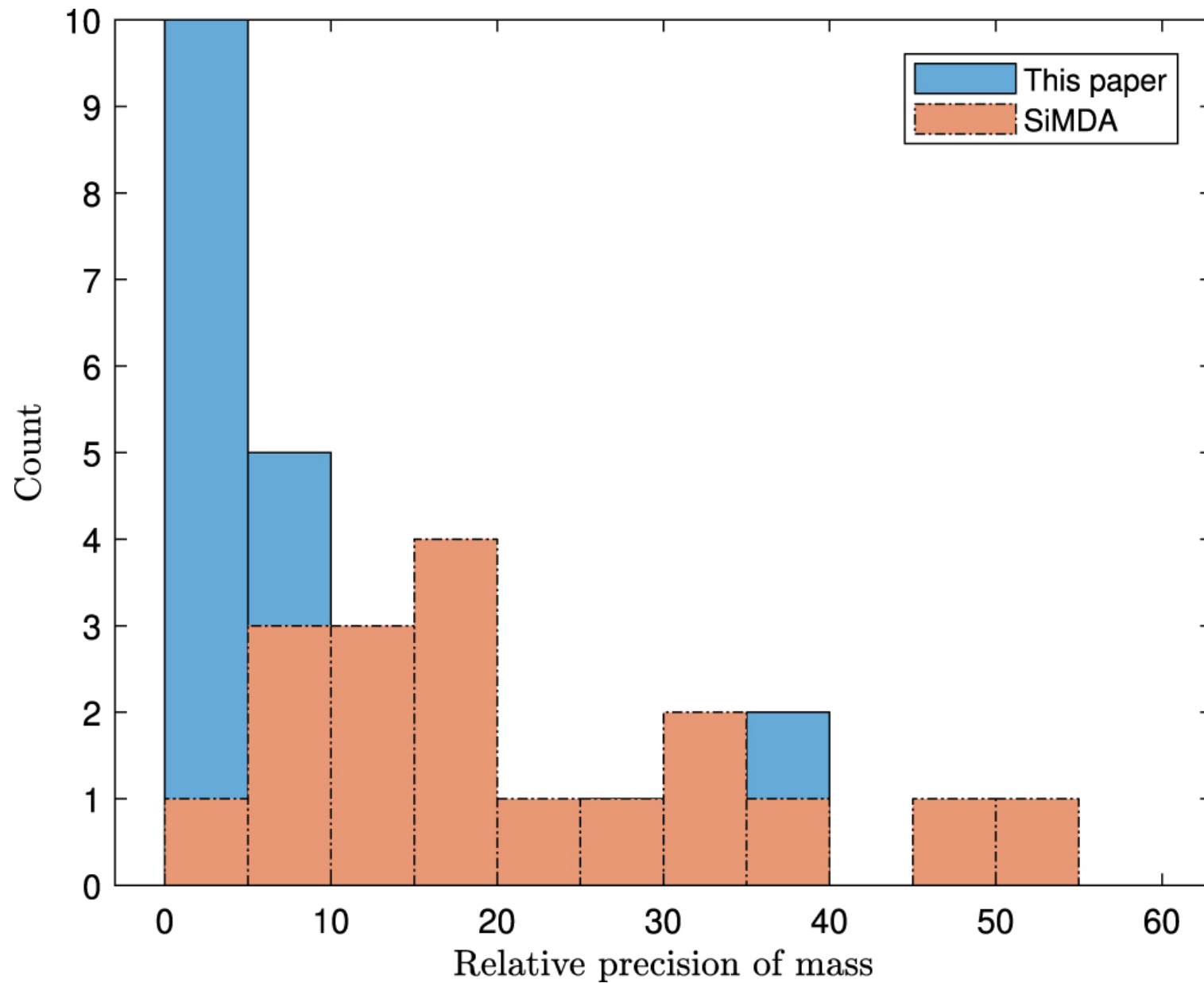
Figure 3. from Fan Li et al 2023 Astron. J. 166 doi:10.3847/1538-3881/ace52b https://dx.doi.org/10.3847/1538-3881/ace52b © 2023. The Author(s). Published by the American Astronomical Society.
