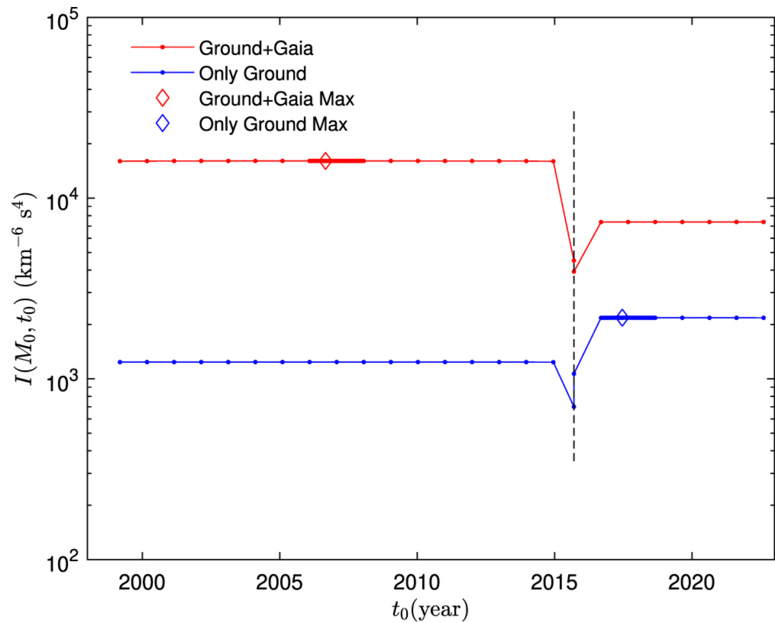
Figure 1. from Fan Li et al 2023 Astron. J. 166 doi:10.3847/1538-3881/ace52b https://dx.doi.org/10.3847/1538-3881/ace52b © 2023. The Author(s). Published by the American Astronomical Society.
