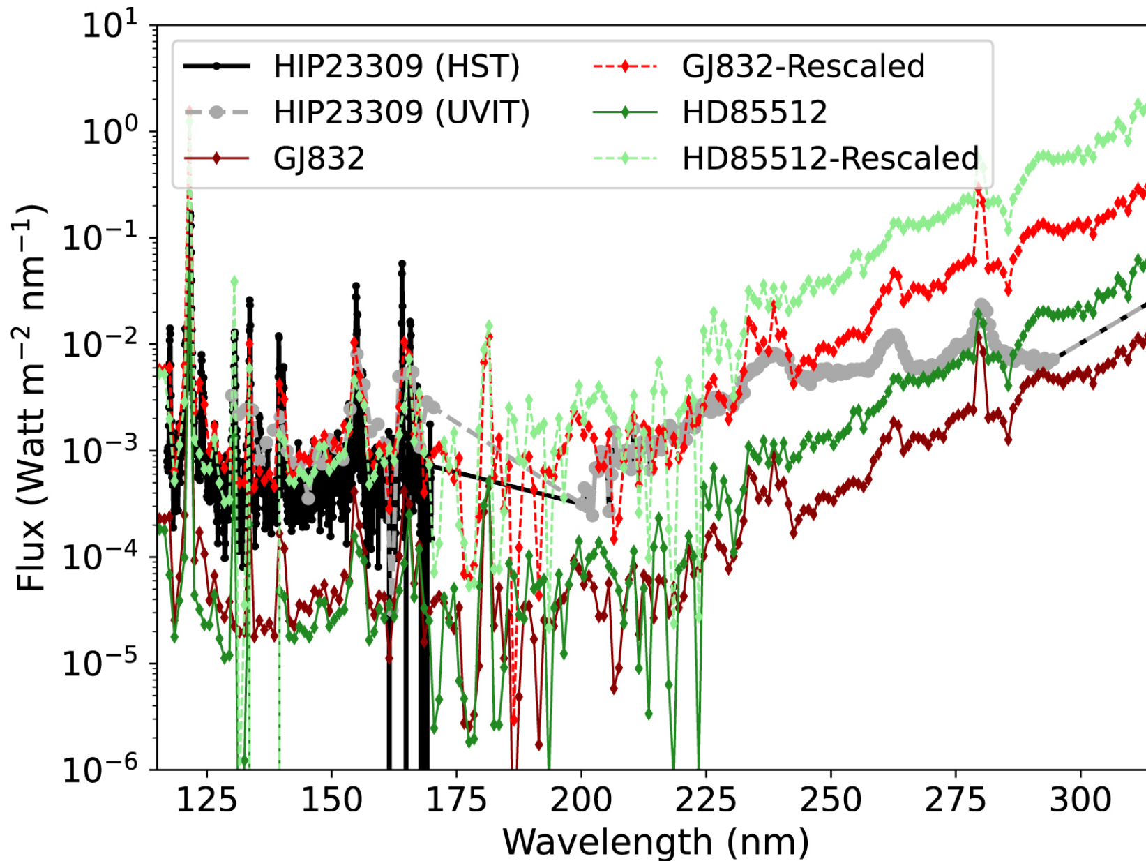
Figure 7. from Sukrit Ranjan et al 2023 Astron. J. 166 doi:10.3847/1538-3881/ace32d https://dx.doi.org/10.3847/1538-3881/ace32d © 2023. The Author(s). Published by the American Astronomical Society.
