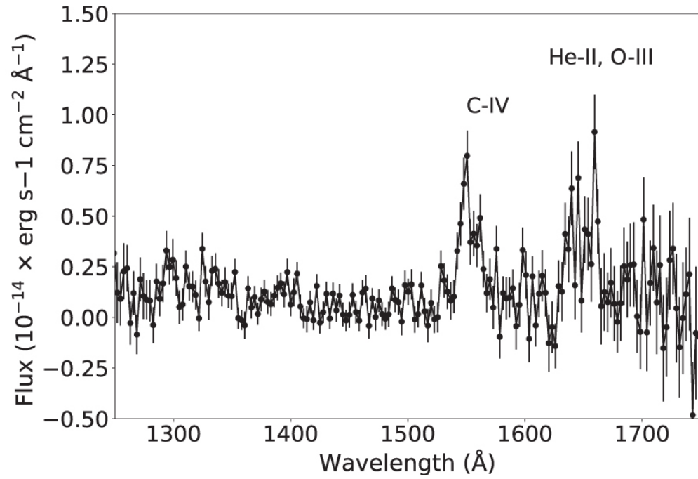
Figure 2. from Sukrit Ranjan et al 2023 Astron. J. 166 doi:10.3847/1538-3881/ace32d https://dx.doi.org/10.3847/1538-3881/ace32d © 2023. The Author(s). Published by the American Astronomical Society.
