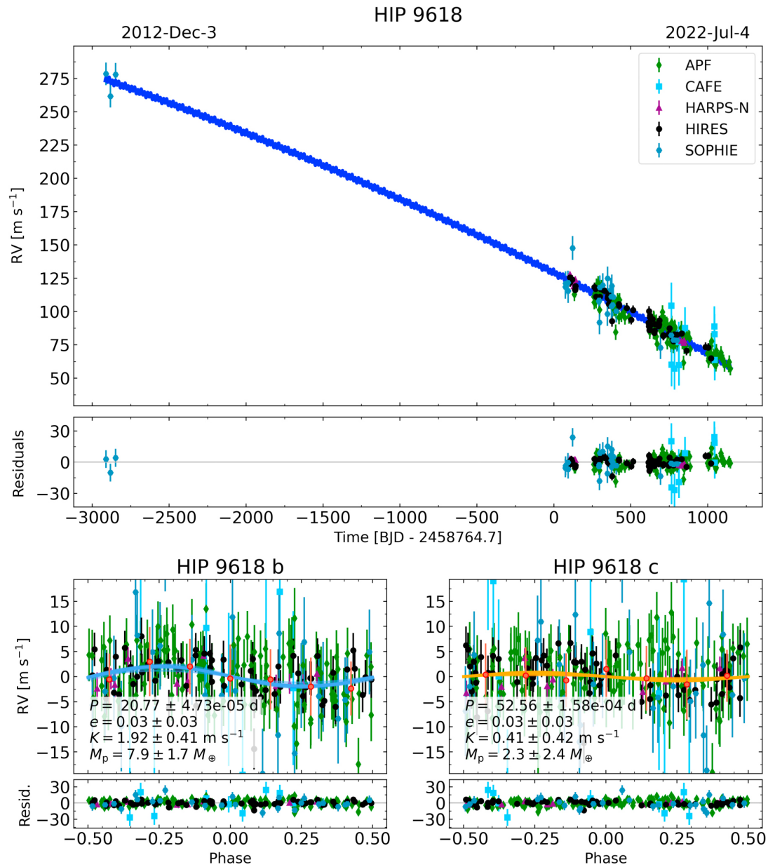
Figure 8. from Joseph M. Akana Murphy et al 2023 Astron. J. 166 doi:10.3847/1538-3881/ace2ca https://dx.doi.org/10.3847/1538-3881/ace2ca © 2023. The Author(s). Published by the American Astronomical Society.
