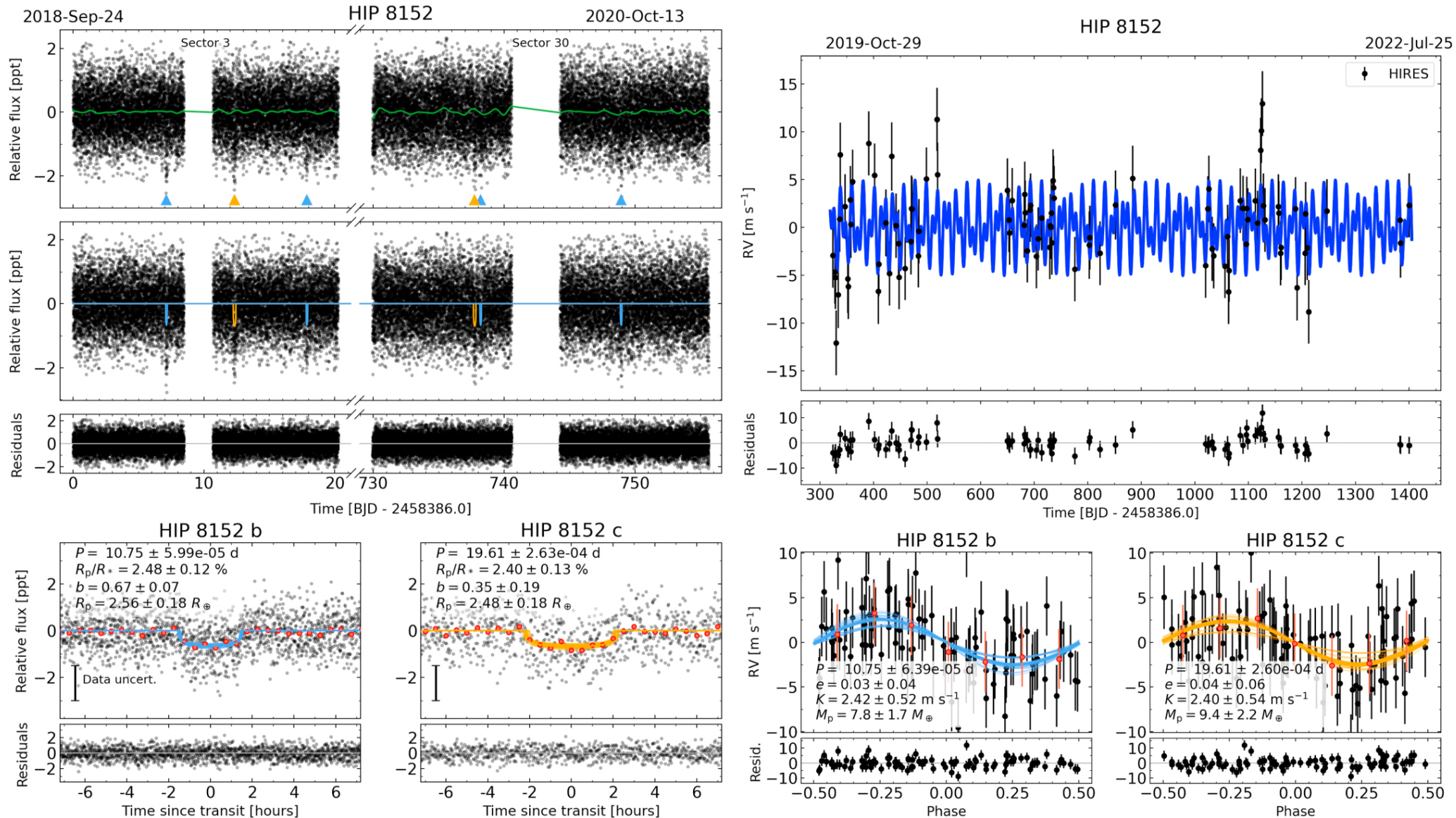
Figure 6. from Joseph M. Akana Murphy et al 2023 Astron. J. 166 doi:10.3847/1538-3881/ace2ca https://dx.doi.org/10.3847/1538-3881/ace2ca © 2023. The Author(s). Published by the American Astronomical Society.
