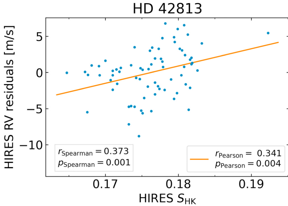
Figure 4. from Joseph M. Akana Murphy et al 2023 Astron. J. 166 doi:10.3847/1538-3881/ace2ca https://dx.doi.org/10.3847/1538-3881/ace2ca © 2023. The Author(s). Published by the American Astronomical Society.
