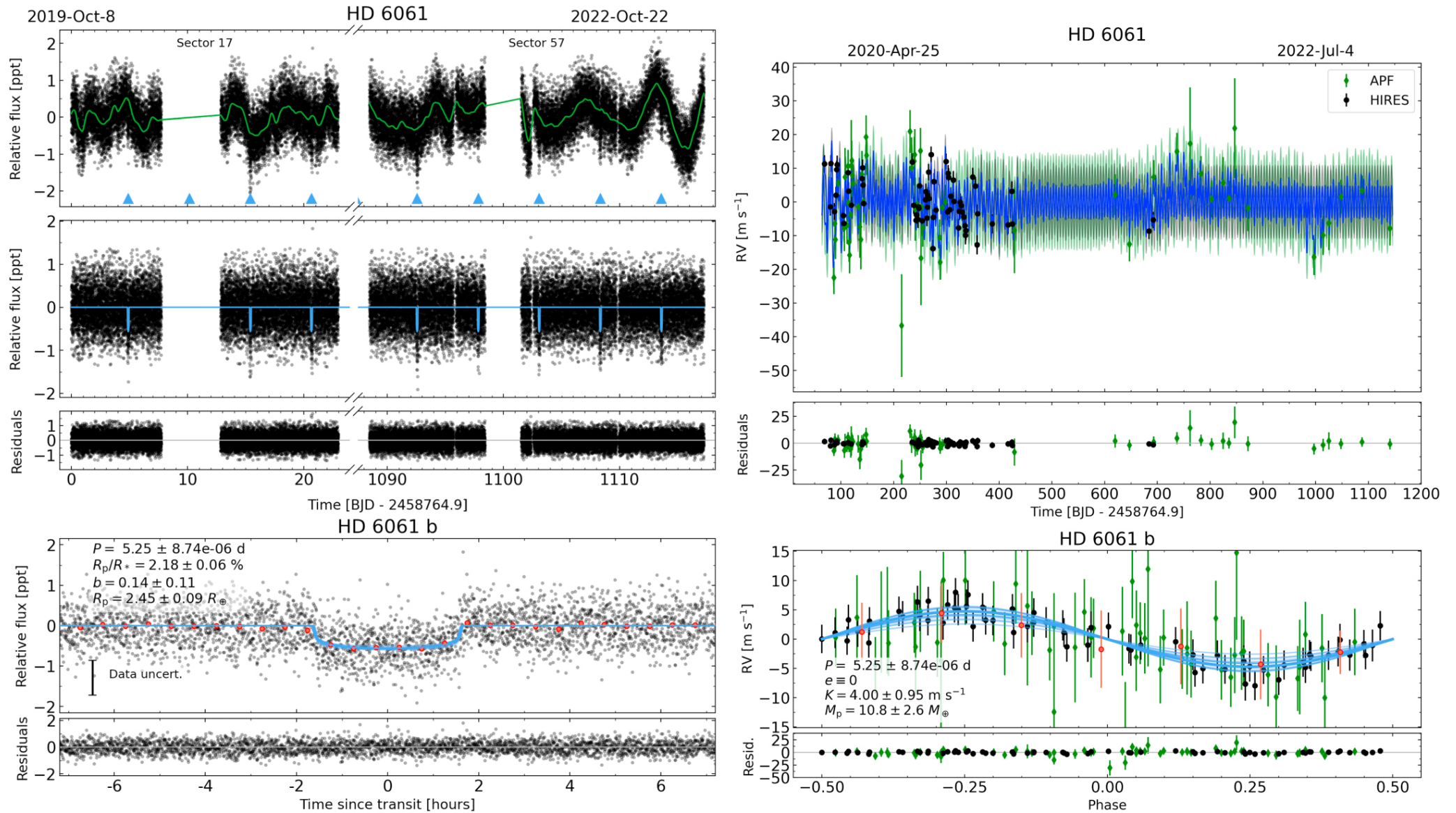
Figure 23. from Joseph M. Akana Murphy et al 2023 Astron. J. 166 doi:10.3847/1538-3881/ace2ca https://dx.doi.org/10.3847/1538-3881/ace2ca © 2023. The Author(s). Published by the American Astronomical Society.
