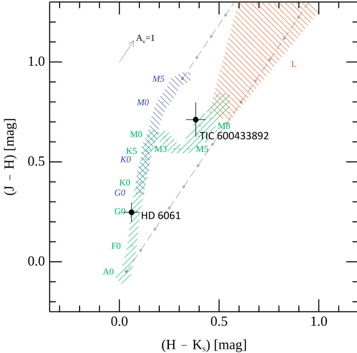
Figure 2. from Joseph M. Akana Murphy et al 2023 Astron. J. 166 doi:10.3847/1538-3881/ace2ca https://dx.doi.org/10.3847/1538-3881/ace2ca © 2023. The Author(s). Published by the American Astronomical Society.
