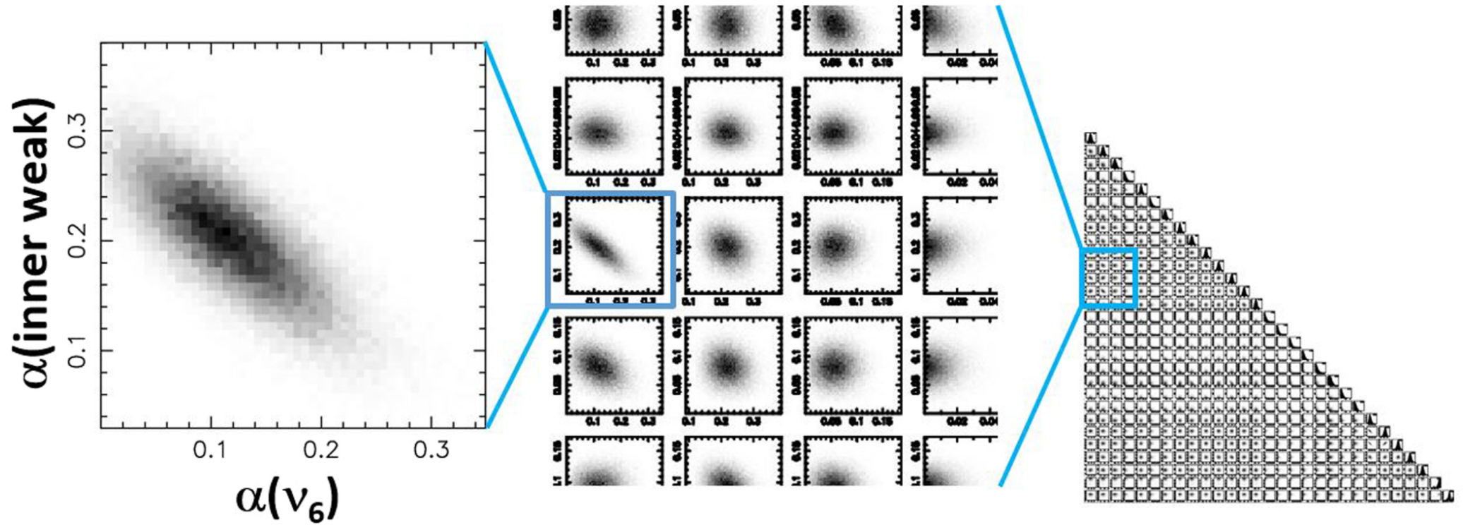
Figure 9. from David Nesvorný et al 2023 Astron. J. 166 doi:10.3847/1538-3881/ace040 https://dx.doi.org/10.3847/1538-3881/ace040 © 2023. The Author(s). Published by the American Astronomical Society.
