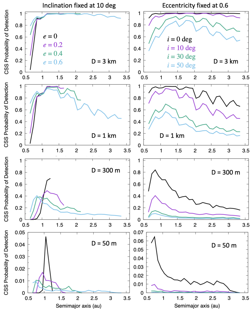
Figure 6. from David Nesvorný et al 2023 Astron. J. 166 doi:10.3847/1538-3881/ace040 https://dx.doi.org/10.3847/1538-3881/ace040 © 2023. The Author(s). Published by the American Astronomical Society.
