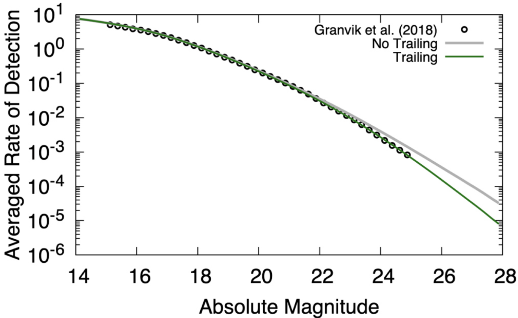
Figure 4. from David Nesvorný et al 2023 Astron. J. 166 doi:10.3847/1538-3881/ace040 https://dx.doi.org/10.3847/1538-3881/ace040 © 2023. The Author(s). Published by the American Astronomical Society.
