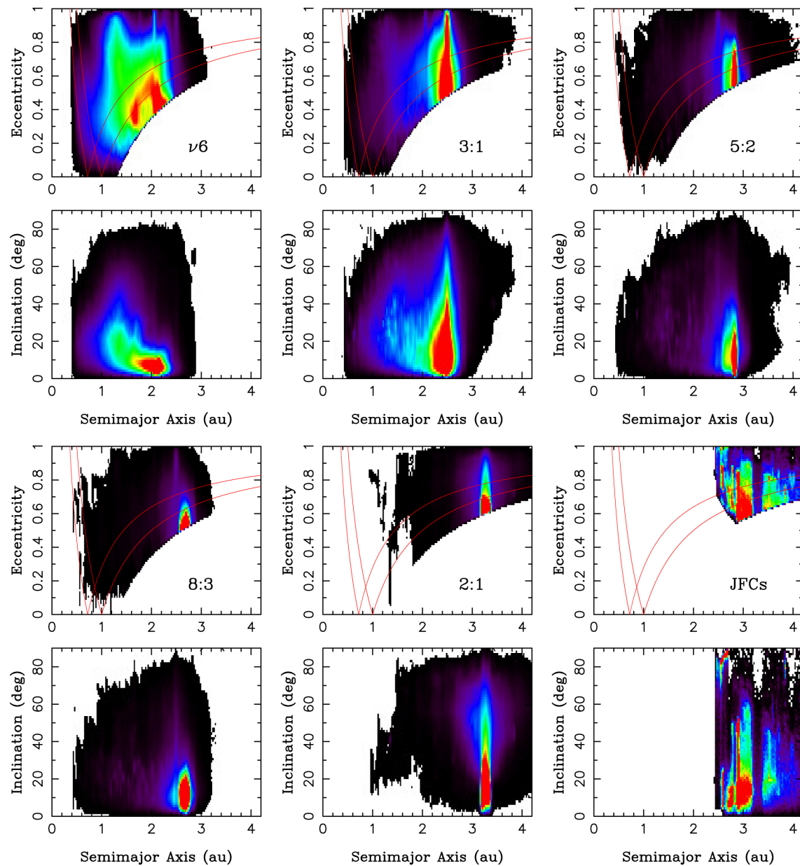
Figure 3. from David Nesvorný et al 2023 Astron. J. 166 doi:10.3847/1538-3881/ace040 https://dx.doi.org/10.3847/1538-3881/ace040 © 2023. The Author(s). Published by the American Astronomical Society.
