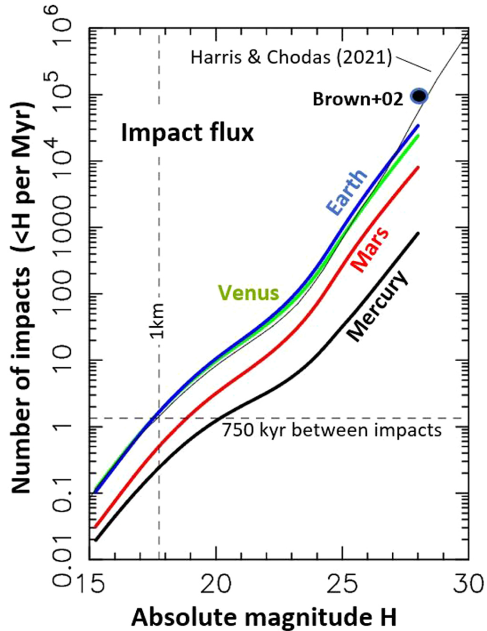
Figure 23. from David Nesvorný et al 2023 Astron. J. 166 doi:10.3847/1538-3881/ace040 https://dx.doi.org/10.3847/1538-3881/ace040 © 2023. The Author(s). Published by the American Astronomical Society.
