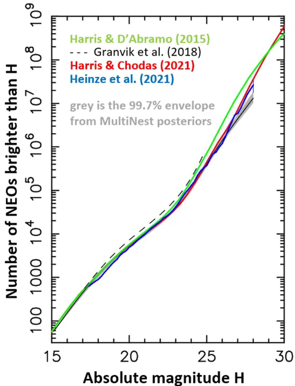
Figure 22. from David Nesvorný et al 2023 Astron. J. 166 doi:10.3847/1538-3881/ace040 https://dx.doi.org/10.3847/1538-3881/ace040 © 2023. The Author(s). Published by the American Astronomical Society.
